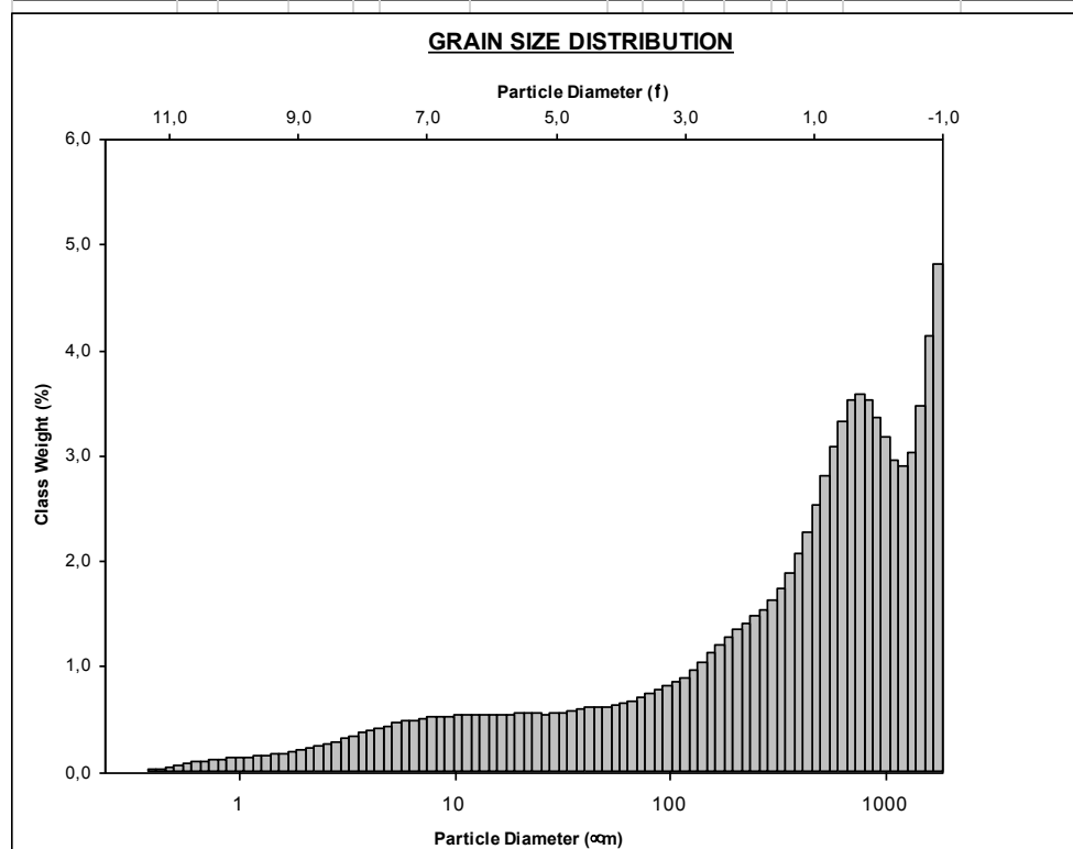
Figur C.2 - Kornfordelingsanalyse SL.
