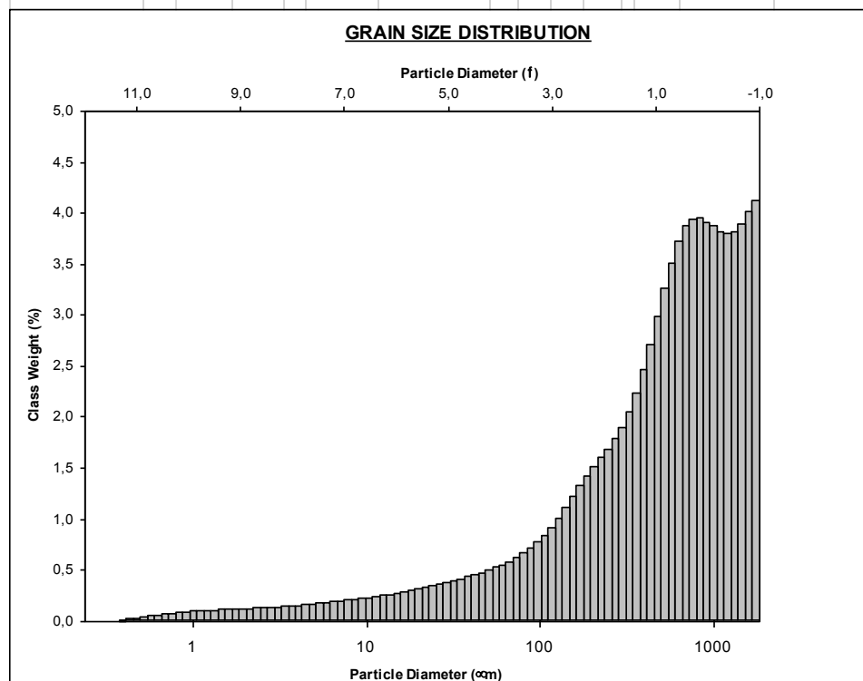
Figur C.3- Kornfordelingsanalyse B.
