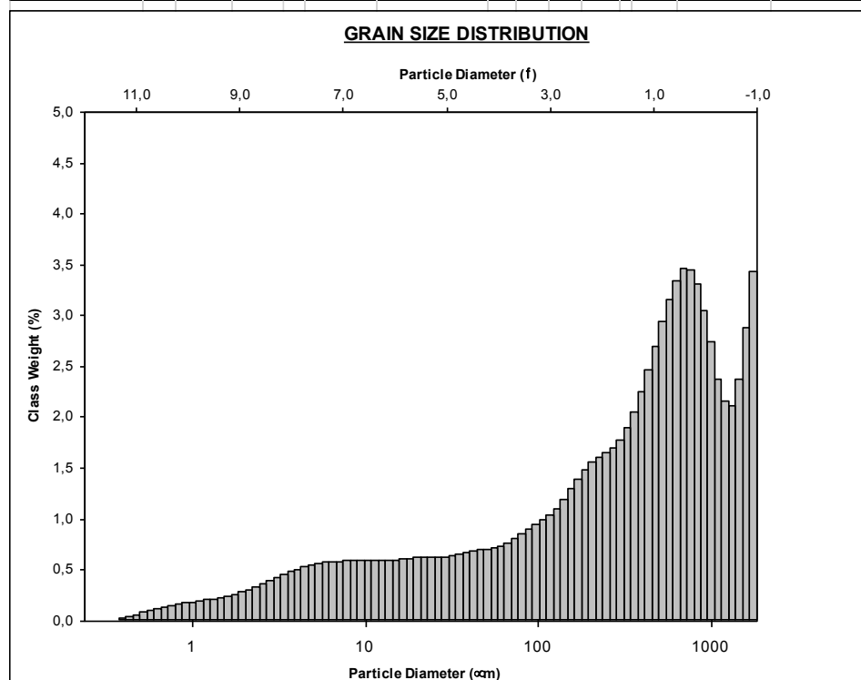
Figur C.1- Kornfordelingsanalyse RE.
