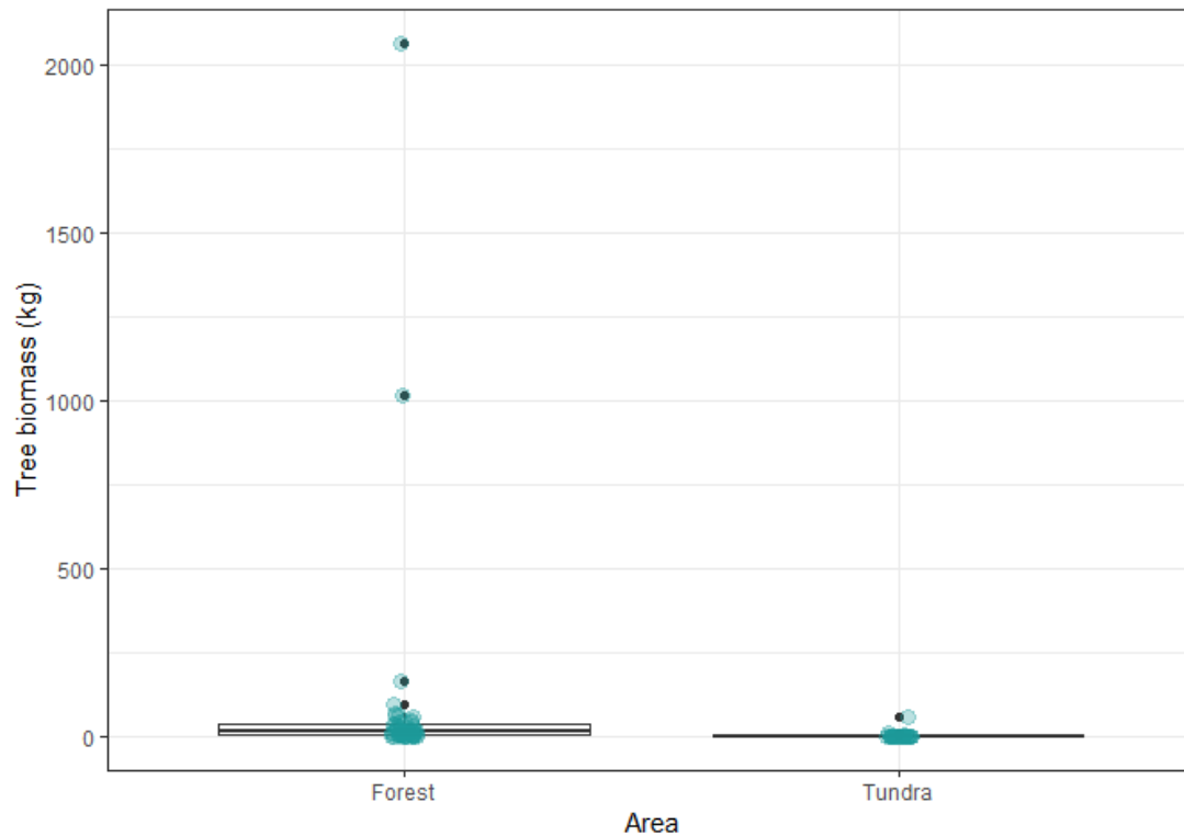
Figure B-1. Boxplots showing average estimated tree biomass, as well as variation in the tree biomass data, in forest compared to tundra for the smallest (radius 4 m) and biggest (radius 10 m) buffer zones.
