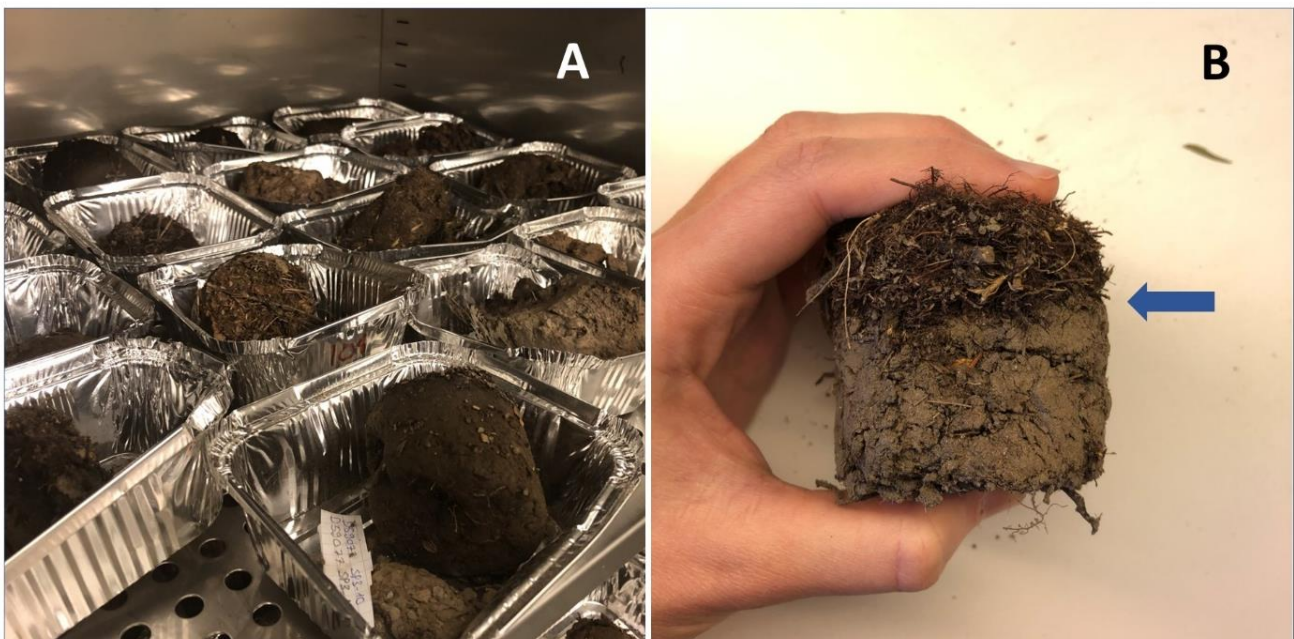
Figure 4. A. Soil samples placed in a drying cabinet to be dried at approximately 40^{\circ}\text{C} before further processing. B. Example of a dried soil sample. The transition between surface soils with high organic matter content (O and A horizons) and mineral soils from beneath the A horizon (marked with arrow), becomes more evident after drying. The deeper mineral soil layers can then be cut off and discarded, and the remaining surface soil sample measured and weighted a final time. Living vegetation was in this case successfully removed prior to the drying. Photograph credits: Claire Devos.
