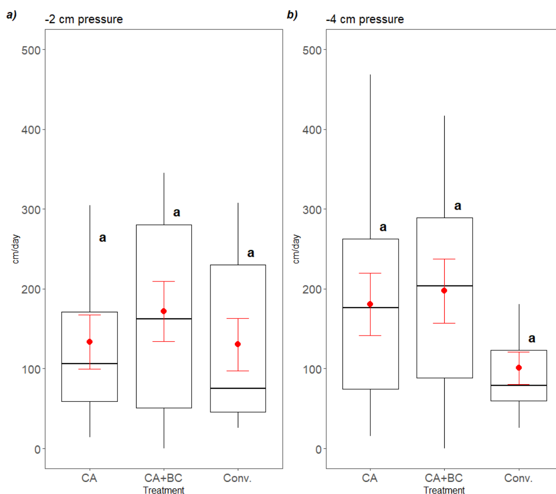
Figure 4: Mean ( \pm standard error) infiltration rate at: a) -2cm pressure ( n=12 each treatment); b) -4 cm pressure ( n=12 each treatment) measured at in-depth experimental site in Alebtong (measurements conducted June 2022) over box-whisker plots (median, 25th and 75th quartile and minimum and maximum values, shown as whiskers). The treatments include conservation agriculture (CA), conservation agriculture + addition of biochar (CA+BC) and conventional practice (Conv.). Letters correspond to significant difference between treatments (Tukey HSD, p -value <0.05 ) within each depth.
