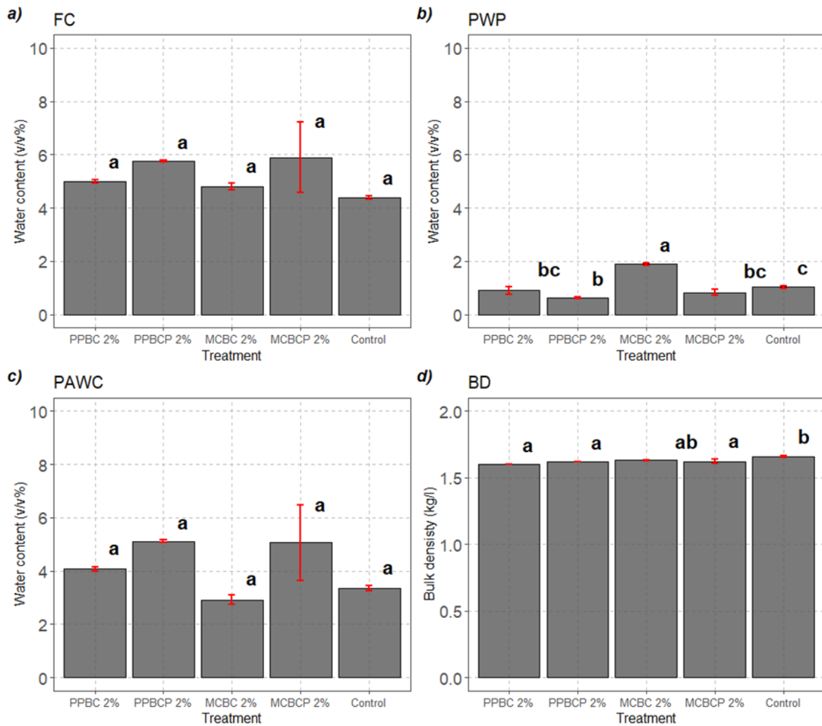
Figure 7: Mean ( \pm standard error) volumetric water content at a) -100cm pressure (FC) ( n=3 each treatment except for MCBCP where n=2 ); b) -15000cm pressure (PWP) ( n=3 each treatment except for MCBCP where n=2 ); c) plant available water content (PAWC) ( n=3 each treatment except for MCBCP where n=2 ); d) bulk density (BD) ( n=3 each treatment except for MCBCP where n=2 ) visualized in bar-plots. Assessing difference in water content between biochar type and particle size for >2 mm particle size, pigeon pea biochar (PPBC); powdered pigeon pea biochar (PPBCP); <2 mm particle size, maize cob biochar (MCBC); powdered maize cob biochar (MCBCP) and >2 mm particle size, sand (Control) in artificially build samples. All samples contain 2 % biochar, by volume. Letters correspond to significant difference between treatments (Tukey HSD, p -value <0.05 ).
