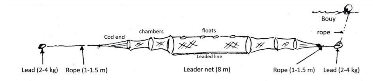
Figure 4. Schematic drawing of a fyke net trap with a leaded leader net, trap chambers and cod ends, all attached to weights, rope, and a buoy.
