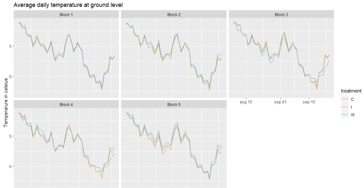
S10: Average daily temperature measurements at ground level. Wet treatment (W) represented with blue lines, intermediate treatment (I) represented with orange lines, and control treatment (C) represented with gray lines.
