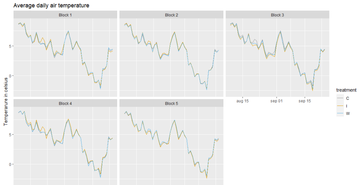
S11: Average daily air temperature measurements, measured at ca. 15 cm above ground level. Wet treatment (W) represented with blue lines, intermediate treatment (I) represented with orange lines, and control treatment (C) represented with gray lines.
