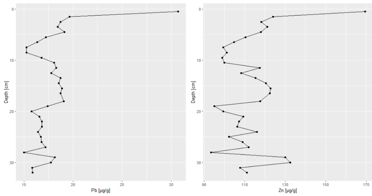
Figure 10 Lead and zinc in \mu\text{g/g} from 0-32 cm depth.
