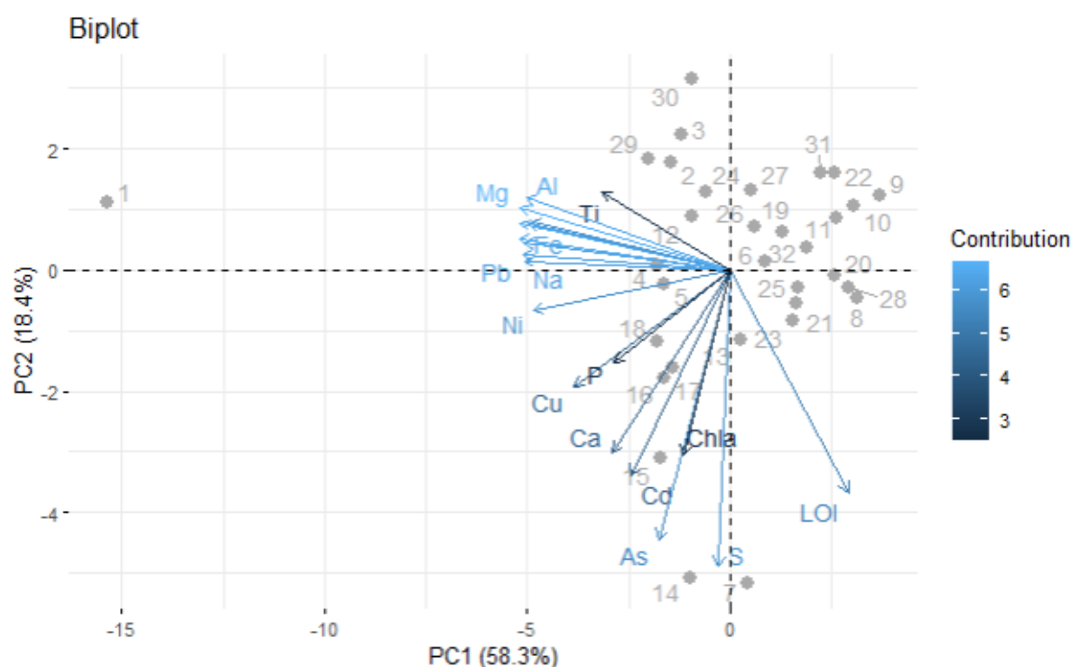
Figure 15 Biplot of first and second principal component from layers S1-S14-S42, S45-S46, i.e., the layers S2-S13 and S43-S44 are excluded. However, the numeric values continue, meaning that S14 corresponds to sample 2, and the last sample 32, corresponds to layer S46. "Chla" stands for chlorophyll a.
