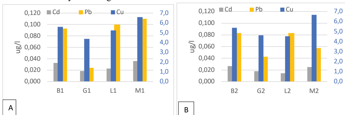
Figure 3.29. Cadmium, Lead and Copper in the drained water from the mesocosm experiment. A soil type 1 and B soil type 2. Cu(blue) is on the right y-axis(µg/l), Cd and Pb on the left y-axis(µg/l).
