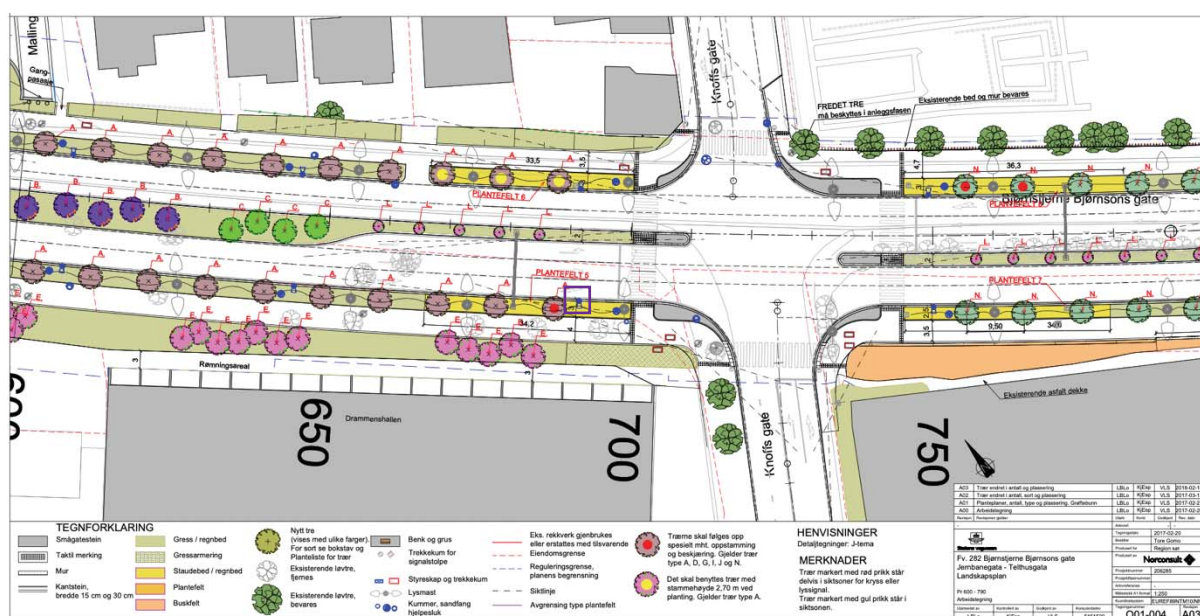
Figure 1.8 Sketch of part of the renovated Bjørnstjerne Bjørnsonsgate. The samples were taken from the manhole(kum) in raingarden 5, indicated with a purple square. (Pers. Med. Kristine Laukli)
