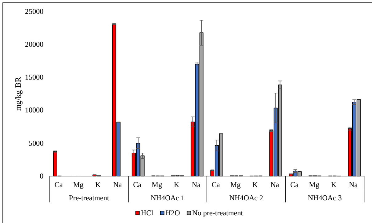
Figure 4. 1: Concentrations of NH 4 OAc-extracted Ca, Mg, K and Na (mg/kg BR) in the pre-treatment extraction, and the three subsequent NH 4 OAc-extractions. Values are means of three triplicates. Error bars indicate standard deviations.
