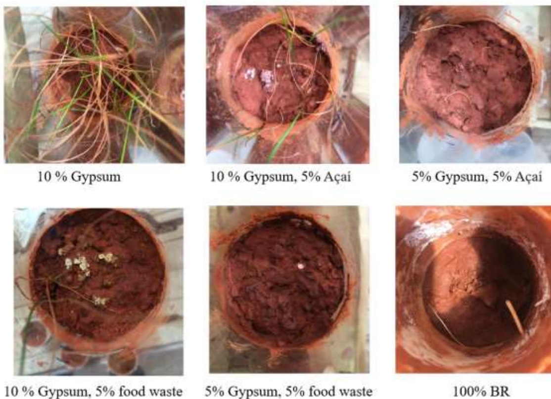
Figure 4.7 Photographs of the germination and development of rye grass, two weeks after seeding. From top left to bottom right. 10% gypsum, 10% gypsum + Açai waste, 5% gypsum + 5% Açai waste, 10% gypsum + 5% food waste and 5% gypsum + 5% food waste.
