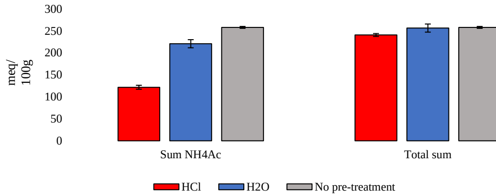
Figure 4. 2: Sum of cations (summed up for the three NH 4 OAc extractions) and total sum of extracted cations (pre-treatment + three NH 4 OAc extractions, indicated as “Total sum”). Values are in meq/100g BR.
