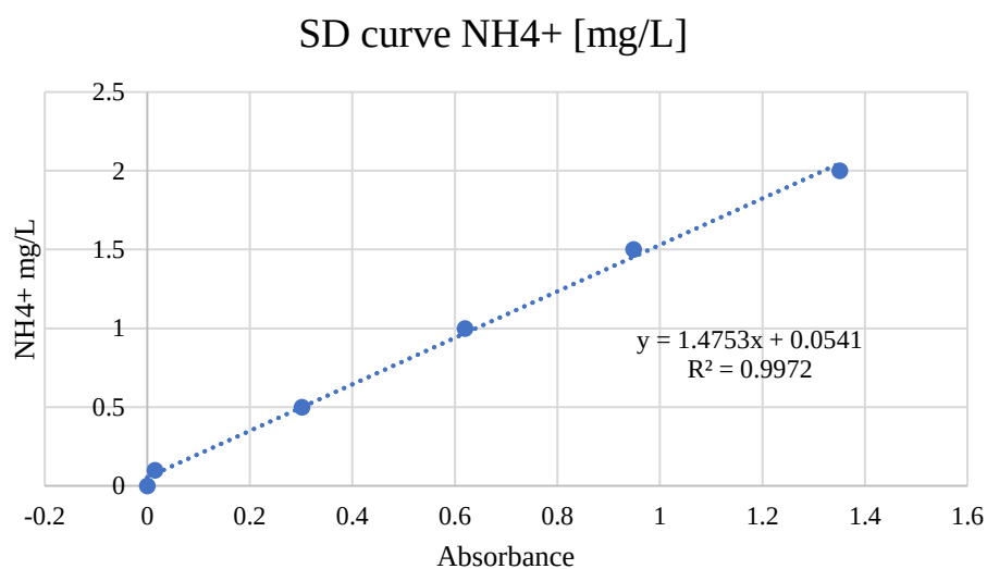
Figure A. 1: SD curve for \text{NH}_4^+ analysis with spectrophotometer. Formula y used to calculate concentrations from absorbance of treatments in table A.3.
