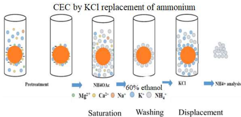
Figure 3. 5 Depiction of the method for determining CEC, based on both 1M \text{NH}_4\text{OAc} (buffered at pH 7) displacement of base cations followed by \text{NH}_4^+ displacement using 2M KCl. Schematic modified from (Munera-Echeverri et al., 2018).
