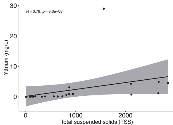
Figure 20: Correlation between total suspended solids (TSS) and yttrium (Y) content in exposed daphnids for the 72 hours test (Kendall: R -value = 0.79, p -value = 8.3e-08).
