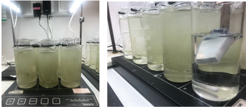
Figures 2 & 3: The photo on the left shows the test setup from the front. The picture on the right shows the other magnetic stirrer board with setup. The HOBO Pendant temperature and light logger is shown in the front on the board. Image: Thea Oma.
