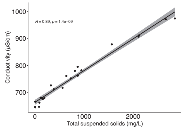
Figure 2: Correlation between conductivity ( \mu\text{S}/\text{cm} ) and total suspended solids (TSS) for the 72 hours toxicity test. (Kendall: R -value = 0.89, p -value = 1.4e-09).
