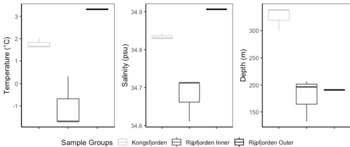
Figure 5 Boxplots of environmental variables. From left temperature, salinity level, and depth measured with CTD at the time of water sample for the three sampling groups: Kongsfjorden, Rijpfjorden Inner and Rijpfjorden Outer. Lower and upper fences are 25th and 75th percentiles, and median is indicated by the bold horizontal line between. Whiskers represent the highest and lowest value.
