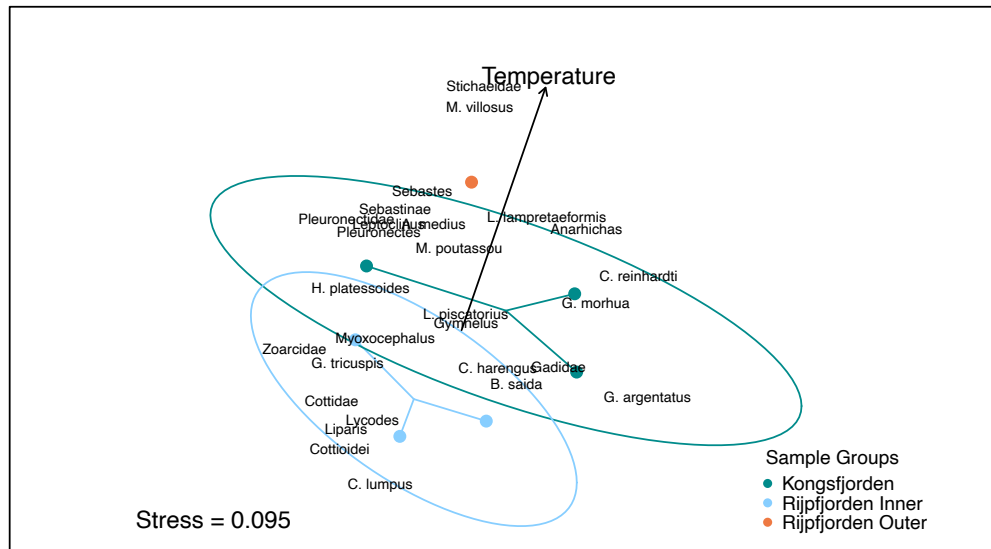
Figure 8 Nonmetric Multidimensional Scaling (NMDS) plot for sampling stations grouped by Kongsfjorden, Rijpfjorden Inner, and Rijpfjorden Outer based on Hellinger transformed abundance data, and Bray-Curtis dissimilarity index with 2 dimensions. Fitted environmental variable, temperature, is represented by black vector. The ellipses represent 95% confidential interval of community composition in NMDS space for each sampling area. Stress value is indicated.
