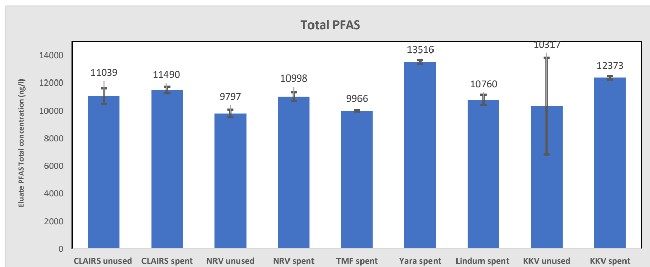
Figure 13: Total PFAS concentration from the control water for the various batch tests. Error bare are included line, (n=3)
