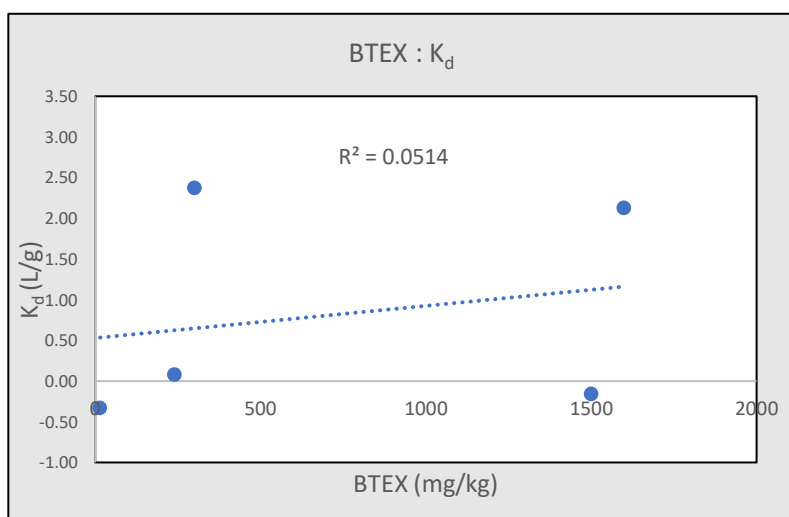
Figure 21a: K_d value and BTEX concentration
