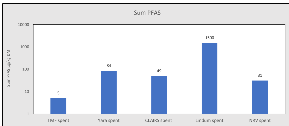
Figure 8: Total concentration of sum PFAS compounds ( \mu\text{g/kg DM} ) from the contamination analysis
