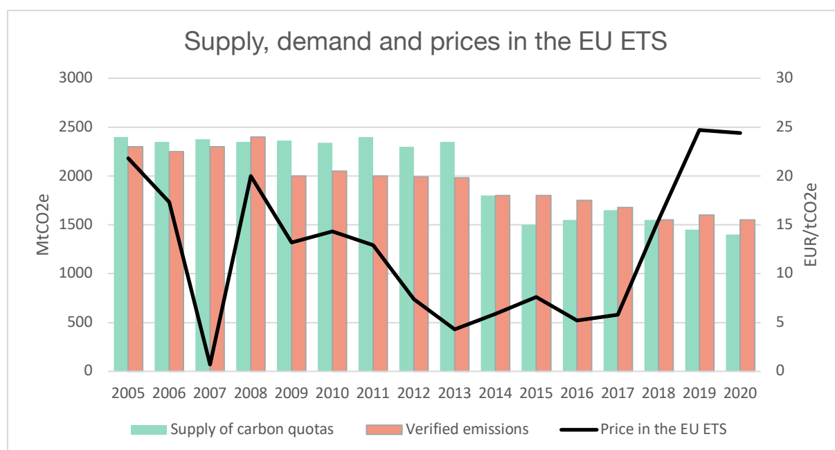
Figure 3: Supply, demand and prices in the EU ETS (European Environment Agency, 2022)
