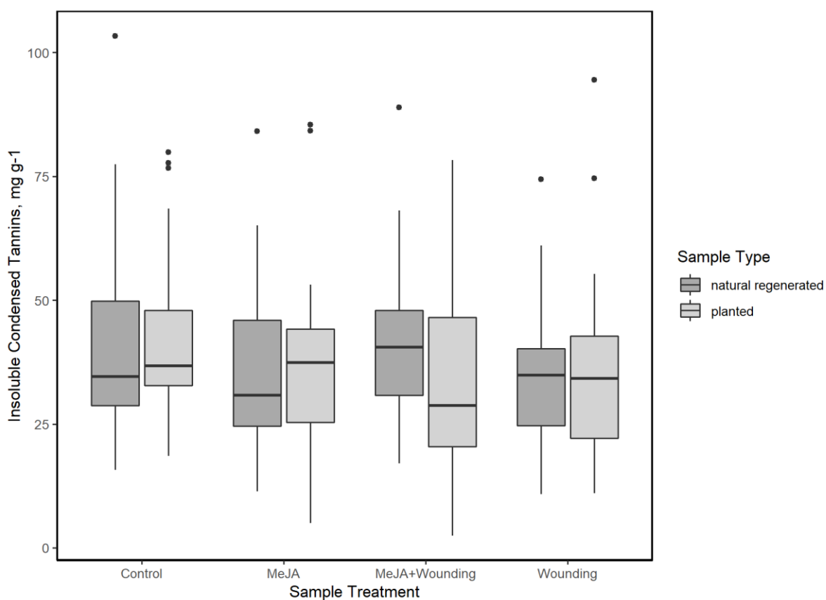
Figure 8: Insoluble condensed tannin concentrations for Norway spruce seedling needles. Differences are displayed between seedling type (naturally regenerated and planted) as well as treatment (MeJA, MeJA+Wounding, Wounding and Control).
