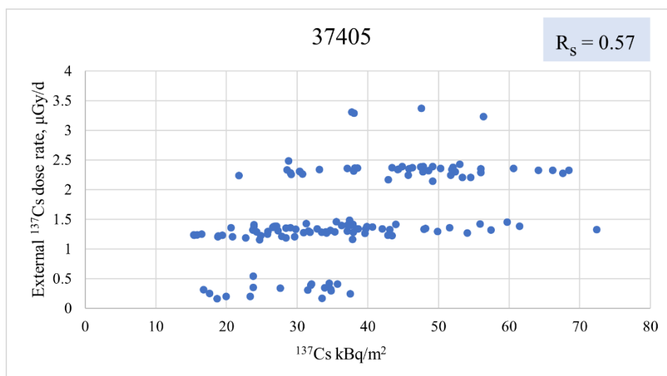
Figure 16: Plot of external ^{137}\text{Cs} dose rates ( n=132 ) registered by GPS-dosimeters and levels of ^{137}\text{Cs} in soil from airborne radiometric survey for reindeer 37405. The Spearman correlation coefficient, r_s , is obtained from a Spearman correlation test. R_s = 0.57 indicate a moderate correlation.
