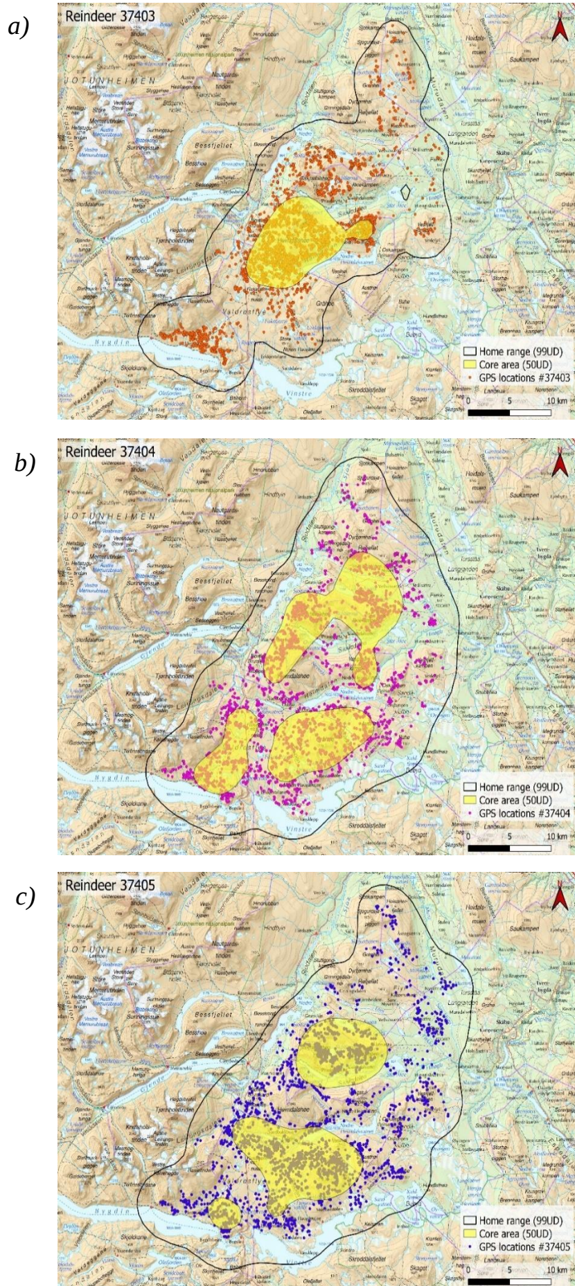
Figure 5: Home range (outlined in black), core area (yellow area(s)), and GPS locations for reindeer 37403 (a), 37404 (b), and 37405 (c). Map data derived from Statens kartverk. (2007). Toporaster WMS. Available as a web map service (WMS) at: http://openwms.statkart.no/skwms1/wms.toporaster4 .
