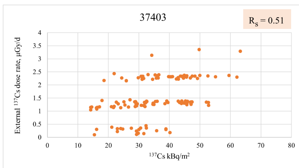
Figure 14: Plot of external ^{137}\text{Cs} dose rates ( n=132 ) registered by GPS-dosimeters and levels of ^{137}\text{Cs} in soil from airborne radiometric survey for reindeer 37403. The Spearman correlation coefficient, r_s , is obtained from a Spearman correlation test. R_s = 0.51 indicate a moderate correlation.
