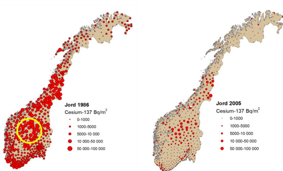
Figure 2: Maps of ^{137}\text{Cs} contamination levels ( \text{Bq/m}^2 ) in soil in Norway. The thesis' study area is highlighted with a yellow circle. The map on the left shows contamination levels in 1986, after the Chernobyl accident. Values vary between 440 and 104 000 \text{Bq/m}^2 . The map on the right shows contamination levels in 2005. Values vary between 120 and 69 000 \text{Bq/m}^2 . Figure derived from Gjelsvik, R., Komperød, M., Brittain, J. E., Eikermann, I. M., Gaare, E., Gwynn, J., Holmstrøm, F., Jensen, L. K., Kålås, J. A., Møller, B., et al. (2014). Radioaktivt cesium i norske landområder og ferskvannssystemer. Resultater fra overvåkning i perioden 1986-2013, 2014:9: Statens strålevern (Norwegian Radiation Protection Authority).
