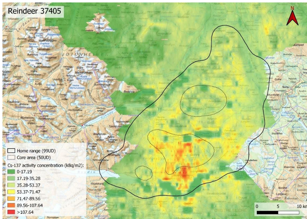
Figure 18: Contamination levels of ^{137}\text{Cs} in home range and core area for reindeer 37405 in 2016. Mapdata derived from: 1) Statens kartverk. (2007). Toporaster WMS. Available as a web map service (WMS) at: http://openwms.statkart.no/skwms1/wms.toporaster4 , 2) NGU (Geological Survey of Norway). (2020). Unpublished.
