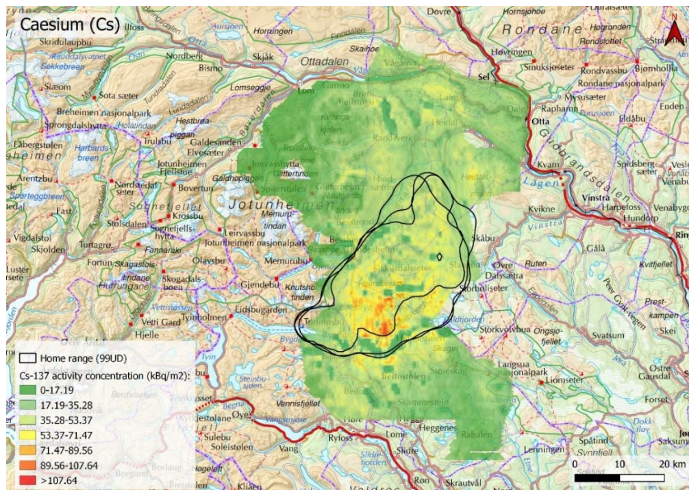
Figure 6: Contamination levels of caesium, ^{137}\text{Cs} , in the herding area (in kBq/m 2 ) as of 2016. Home ranges of the reindeer are outlined in black. Contamination levels are not decay corrected but do still represent the distribution of ^{137}\text{Cs} in the area. Mapdata derived from: 1) Statens kartverk. (2007). Toporaster WMS. Available as a web map service (WMS) at: http://openwms.statkart.no/skwwms1/wms.toporaster4 , 2) NGU (Geological Survey of Norway). (2020). Unpublished.
