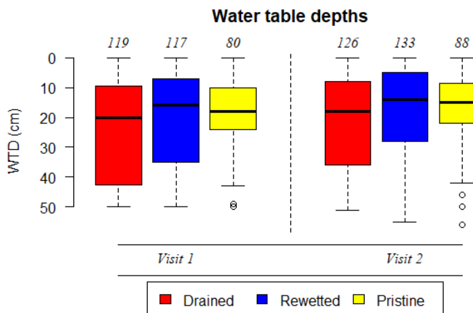
Figure 5. Box-whisker plot of specific water table depth (WTD) measurements on drained (red), rewetted (blue), and pristine bogs (yellow). The boxes cover 66% of measurements ( \pm 1 standard deviation (SD) from the mean); whiskers indicate 95 % confidence interval ( \pm 2 SD); medians are indicated by thick solid horizontal line. Dots indicate single outliers. Numbers above the boxes indicate sample sizes.
