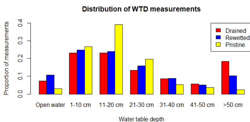
Figure 6. Distribution of measurements of water table depths, sorted by mire treatment. There were more instances of hitting no water at 50 cm depth on the drained mires than on either of the other two treatments. Pristine mires had less open water, but more water close to the surface than the other treatments. There was also greater variation in measurements on rewetted and drained sites.
