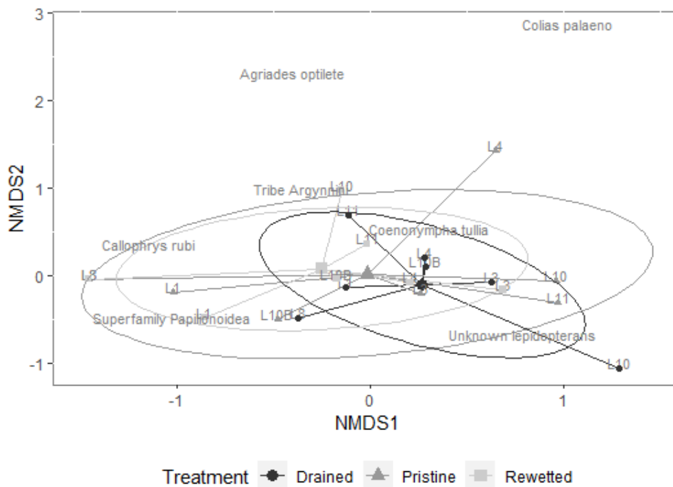
Figure 5: A two dimensional NMDS of the butterfly community in drained, rewetted and pristine bogs. The ellipses represent 1 SD and spider webs connect and draw the centroids for each of the three treatments in every location. None of the treatments were significantly different from one another.
