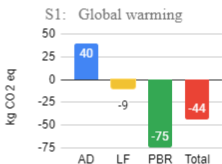
Figure 17: Results of GWP of Scenario 1.
