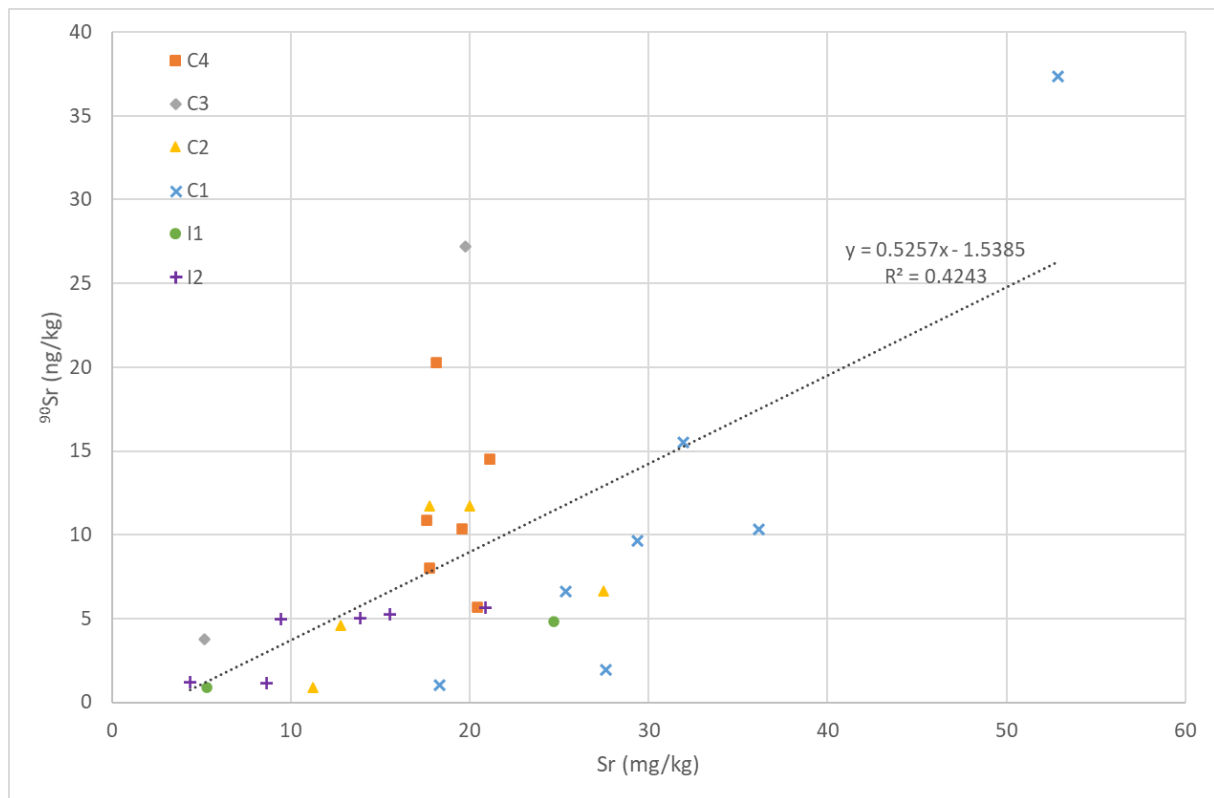
Figure 3.3: Scatter plot of the Sr vs. ^{90}\text{Sr} concentrations of the analysed Chernobyl arthropods from six sites. Site C4 (orange), C3 (grey), C2 (yellow), C1 (blue), I1 (green) and I2 (purple).
