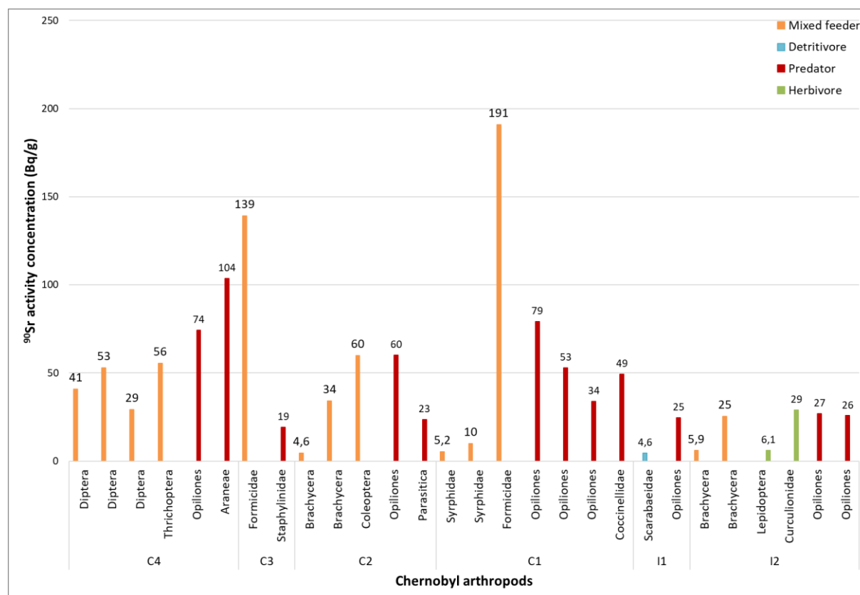
Figure 3.1: Strontium-90 activity concentrations determined in analysed Chernobyl arthropods compared between collection site and trophic level. Mixed feeder (orange), Detritivore (blue), Predator (red) and Herbivore (green).
