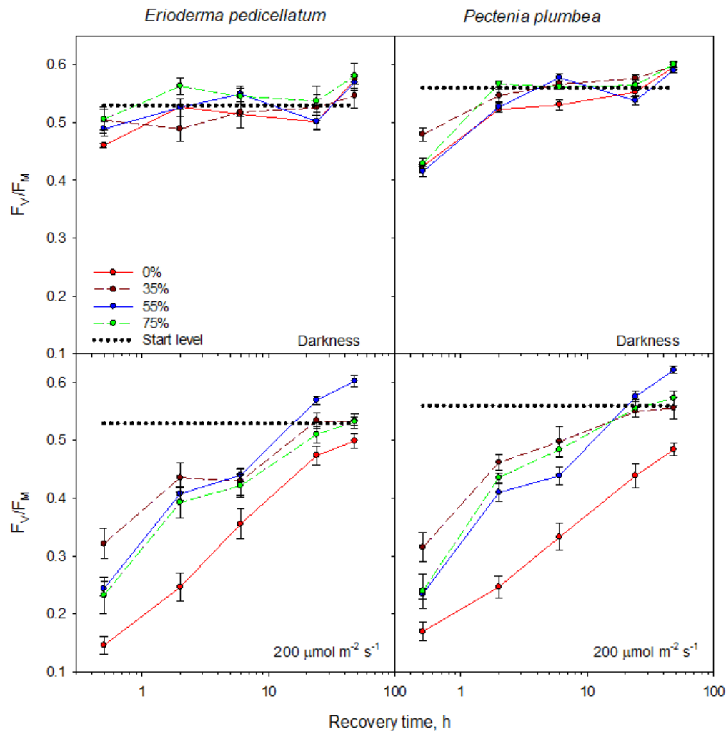
Fig. 17 F_v/F_m kinetics during recovery (h) after 7 d exposure to four levels of relative humidity and two light levels (0 and 200 \mu\text{mol photons m}^{-2} \text{s}^{-1} ), x-axis is log-scale, and dotted lines represent mean start level. Vertical bars show \pm 1 standard error. ( E. pedicellatum n=80 , P. plumbea n=64 )
