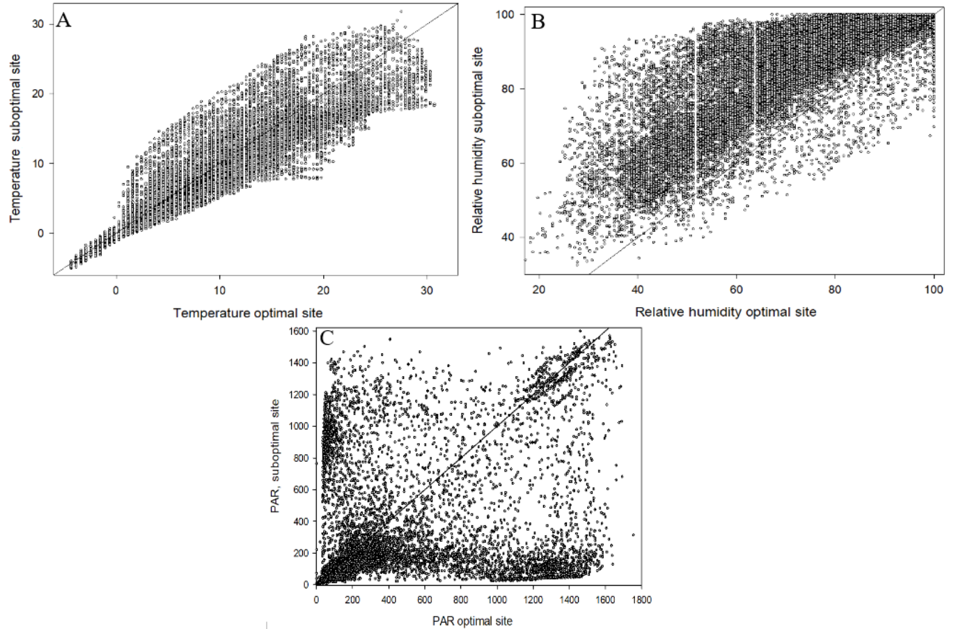
Fig. 10 (A) Temperature (°C), (B) relative humidity (RH, %) and (C) photosynthetic active radiation (PAR, \mu\text{mol photons m}^{-2} \text{s}^{-1} ) for both the optimal and suboptimal site of E. pedicellatum at Tegningfallet, respectively, plotted against each other. A line showing equal values are shown.
