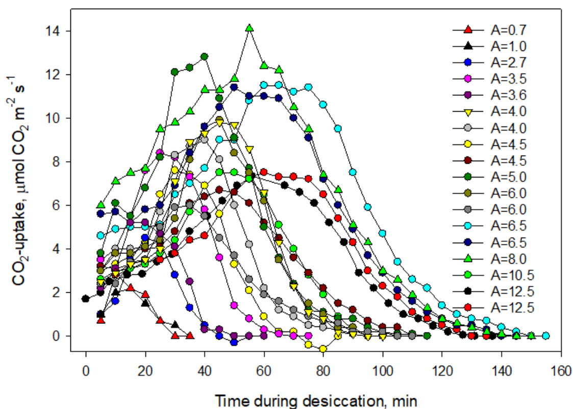
Fig. 14 CO_2 -uptake ( \mu mol CO_2 m^{-2} s^{-1} ) during a desiccation cycle for E. pedicellatum ( n=18 ), with time during desiccation in minutes on x-axis. Legends show thallus area ( cm^2 ) for each thallus, represented with colour/shape.
