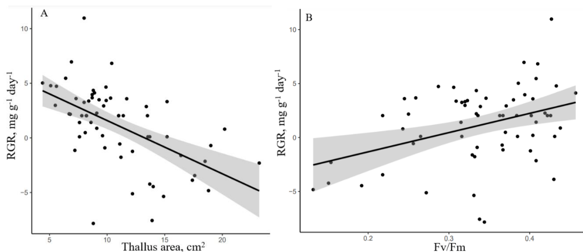
Fig. 19 (A) Relationship between relative growth rate (RGR) and thallus area for E. pedicellatum , R^2_{\text{adj}} = 0.297 , P < 0.001 . (B) The relationship between relative growth rate (RGR) and Fv/Fm, R^2_{\text{adj}} = 0.129 , P = 0.002 . Regression lines (solid lines) and 95% confidence intervals (grey areas) are given.
