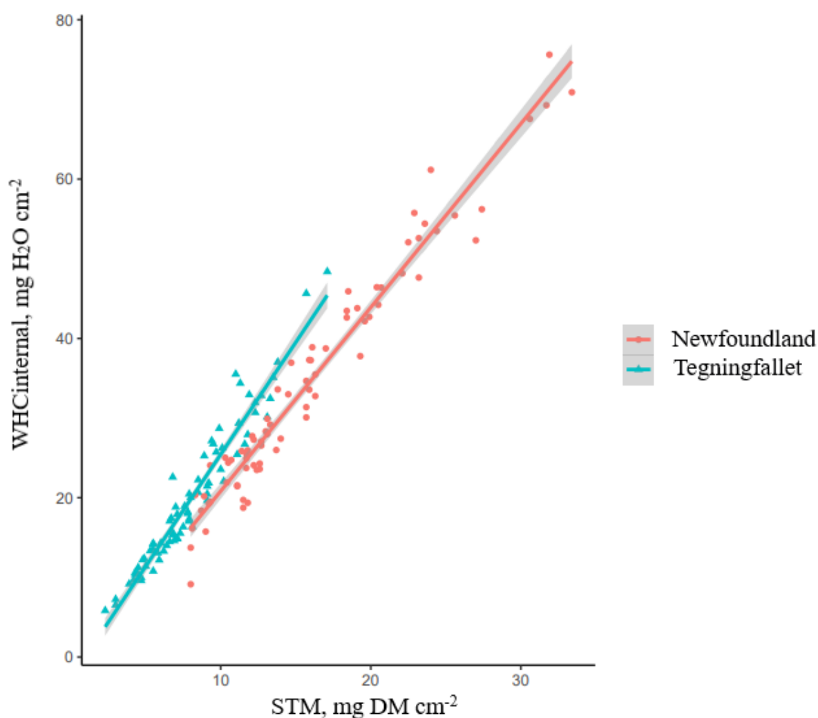
Fig. 20 The relationship between internal water holding capacity ( WHC_{internal} ) and specific thallus mass (STM) for the Newfoundland ( R^2_{adj} = 0.956 , P < 2.2e-16 ) and Tegningfallet ( R^2_{adj} = 0.935 , P < 2.2e-16 ) populations, respectively. (Circles represent Newfoundland, Canada; triangles represent Tegningfallet, Norway.) Regression equations: Tegningfallet: WHC_{internal} = -2.678 + 2.812 * STM ; Newfoundland: WHC_{internal} = -2.227 + 2.306 * STM . Regression lines (solid lines) and 95% confidence intervals (grey areas) are given.
