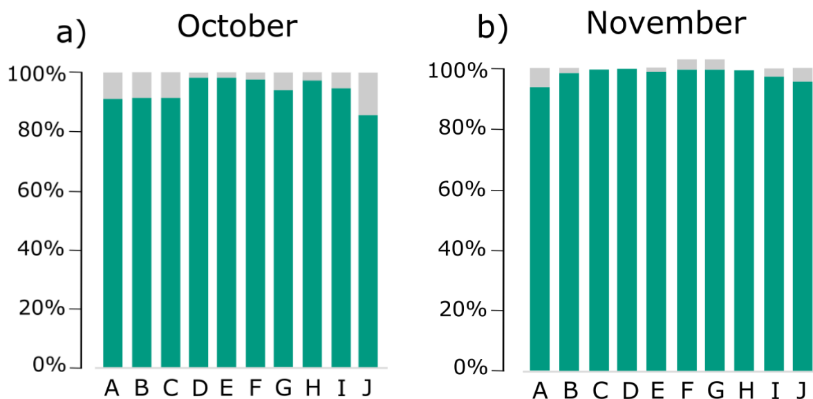
Figure 10 The size distribution (in %) between green: dissolved organic carbon (DOC) ( < 0.2 \mu\text{m} ) and grey: particulate organic carbon (POC) ( > 0.2 \mu\text{m} ) during a) the October sampling and b) the November sampling.
