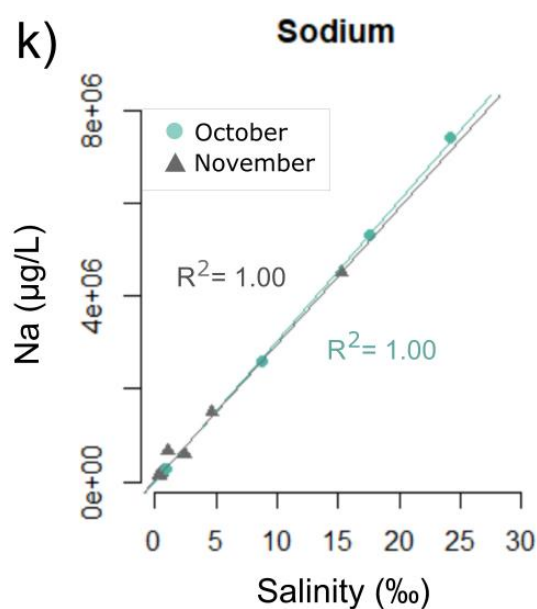
Figure 11k Correlation between sodium (Na) and salinity along the river-ocean transect Storelva – Sandnesfjorden.
