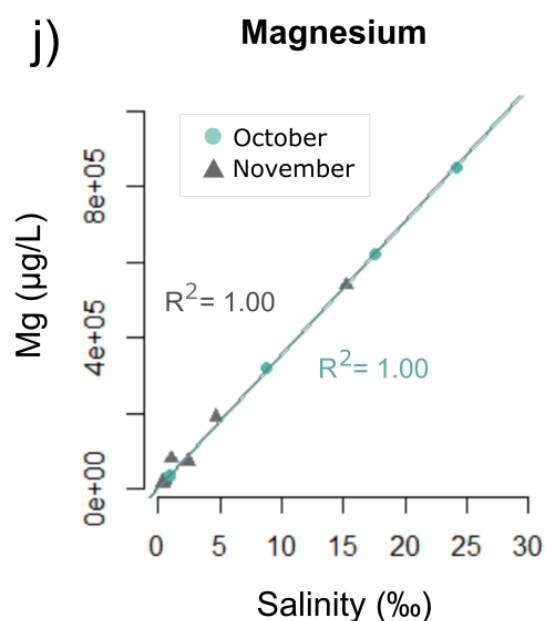
Figure 11j Correlation between magnesium (Mg) and salinity along the river-ocean transect Storelva – Sandnesfjorden.
