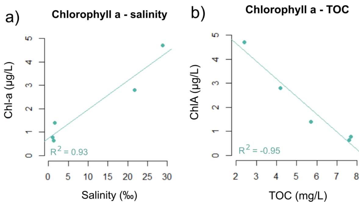
Figure 13 Correlation between a) chlorophyll a (chl-a) and salinity and b) chl-a and total organic carbon (TOC) along the river-ocean transect Storelva-Sandnesfjorden.
