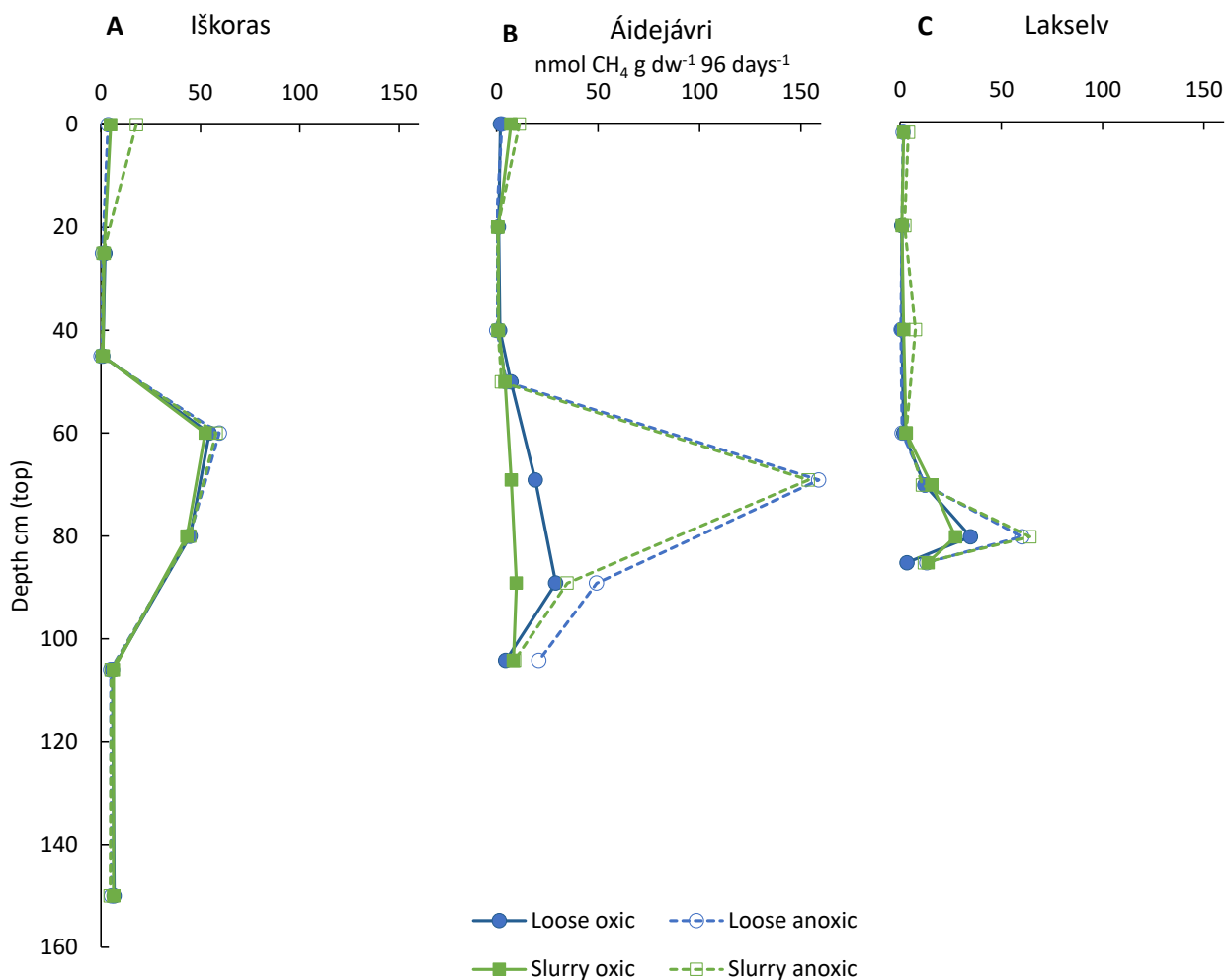
Figure 42: Cumulative CH 4 over depth and 96 days under different incubation conditions (treatments). Stipulated lines indicate the position of the data points in the peat profile as AL (AL1, AL2 and AL3), TZ and PF (PF1, PF2 and PF3). A: Iškoras. B: Áidejávri. C: Lakselv
