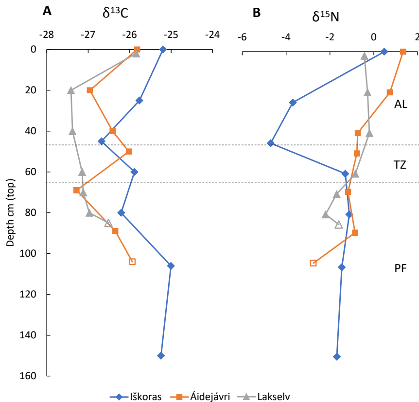
Figure 23: Depth profiles of stable isotopes ratios ( \delta^{13}\text{C} and \delta^{15}\text{N} ) at the three sites. A: ^{13}\text{C}/^{12}\text{C} ratio. B: ^{15}\text{N}/^{14}\text{N} ratio. Hollow markers are mineral soil
