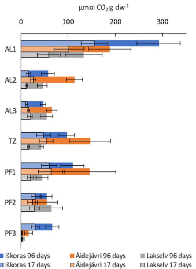
Figure 35: Cumulative CO 2 production averaged across incubation treatments (oxic, anoxic, loose, slurry) in different layers. Shown are stacked values for 17 and 96 days of incubation. Error bars are SE
