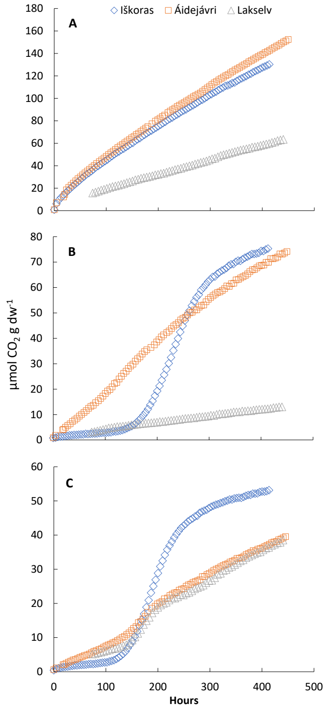
Figure 31: Comparison of CO 2 kinetics over 19 days across sites for the treatment loose oxidic. A: Top active layer (AL1). B: Transition zone (TZ). C: Middle permafrost layer (PF2). Initial data for Lakselv are missing due to instrument failure. Note different scales on y-axis
