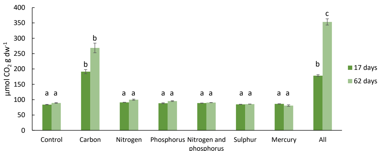
Figure 39: Average (n=3) CO 2 production of Iškora PF2 after 17 and 62 days of incubation in the presence of nutrients. Error bars are SE. Different letters denote statistically significant differences between treatments
