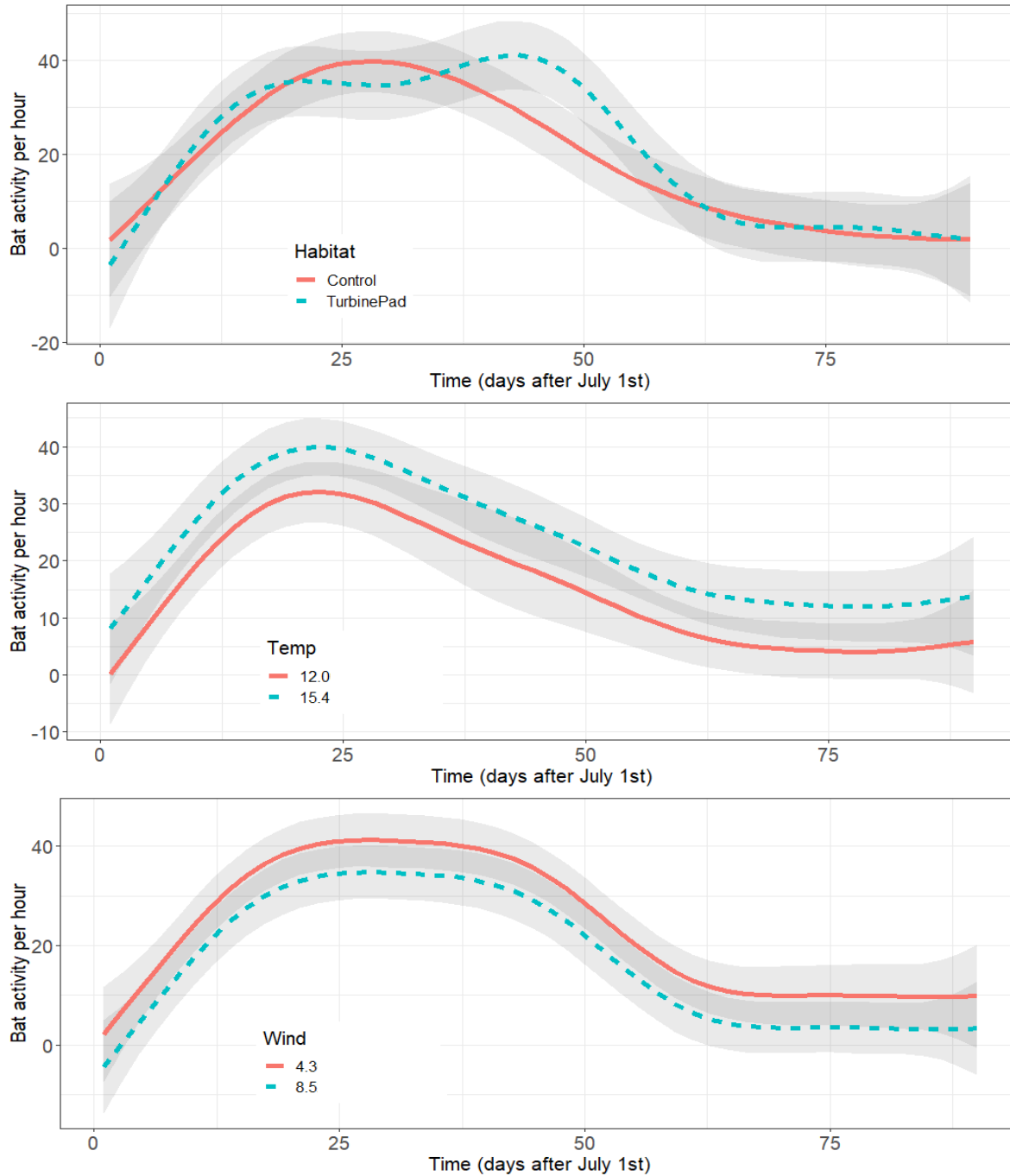
Figure 14. Top(a). Predicted temporal pattern in bat activity at each ground-level habitat type (turbine pads and control sites). Estimated relationships and associated 95% confidence intervals for the GAM model M1b in Table 8. Middle(b). Predicted temporal pattern in bat activity over the course of the study period at different temperatures (2nd and 4 th quantiles). Temp is the average temperature per night, in Celsius, from kl. 22 in the evening until kl. 04 in the morning. Bottom(c). Predicted temporal pattern in bat activity over the course of the study period at different wind speeds (2nd and 4 th quantiles). Wind is the average wind speed (m/s=meters per second) per night from kl. 22 in the evening until kl. 04 in the morning. The common x-axis are the days of the study period beginning July 1 st (day 1) and ending on September 29 th (day 91).
