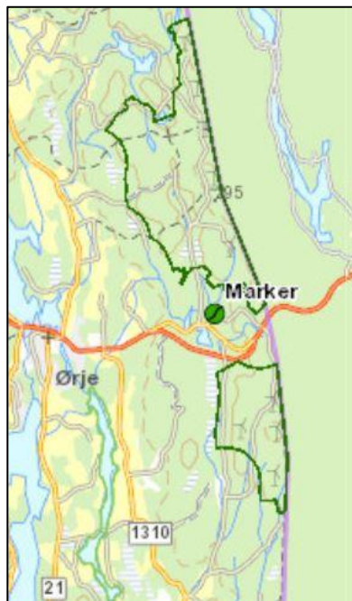
Figure 1. Maps indicate the location of the north and south wind facility (a) and the study area location within Norway (b). Images sourced from NVE.no (a) & Norgeskart.no (b).
