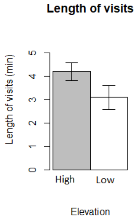
Figure 8: Bar graph showing the length of insect visits observed per flower at the two sites on Sandalsnuten, Finse, with 95% confidence intervals.
