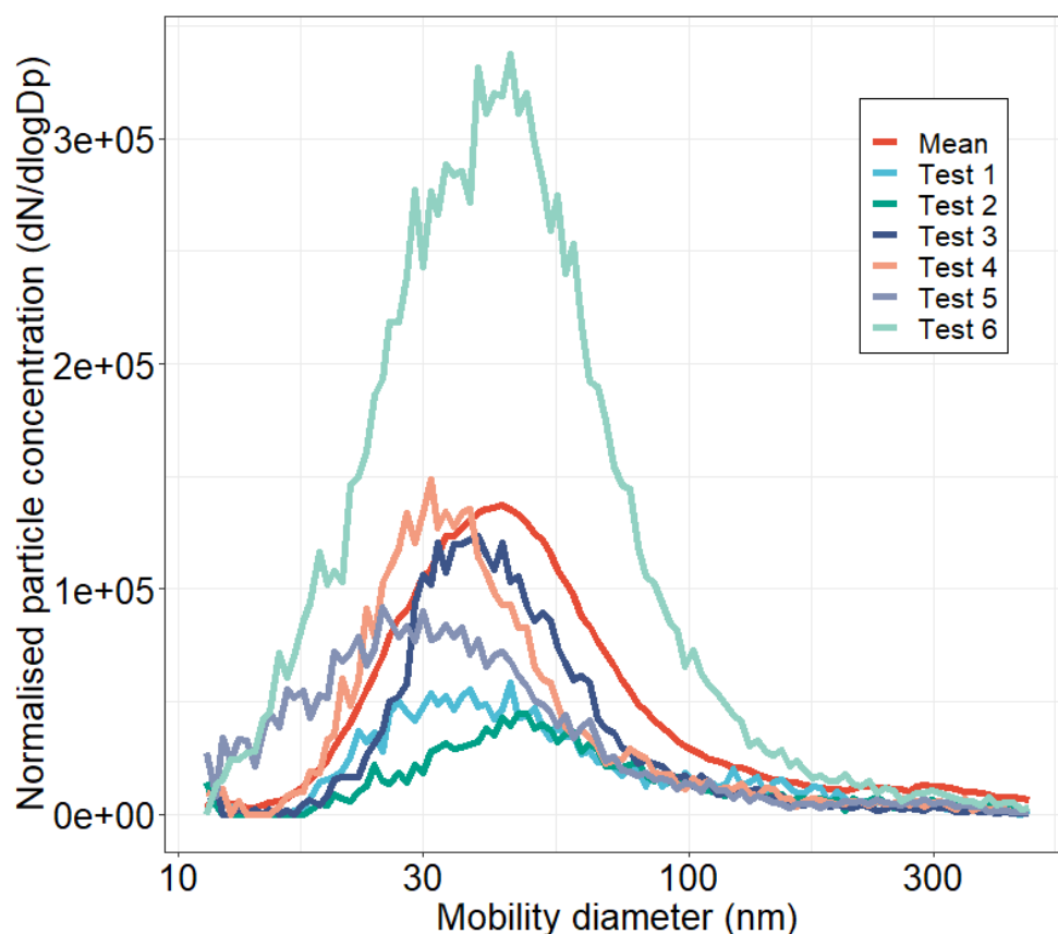
Figure S4.1 Comparing six tests of two consecutive measurements from SMPS with the overall mean of 91 measurements on the same material (Stainless steel 6 mm).
