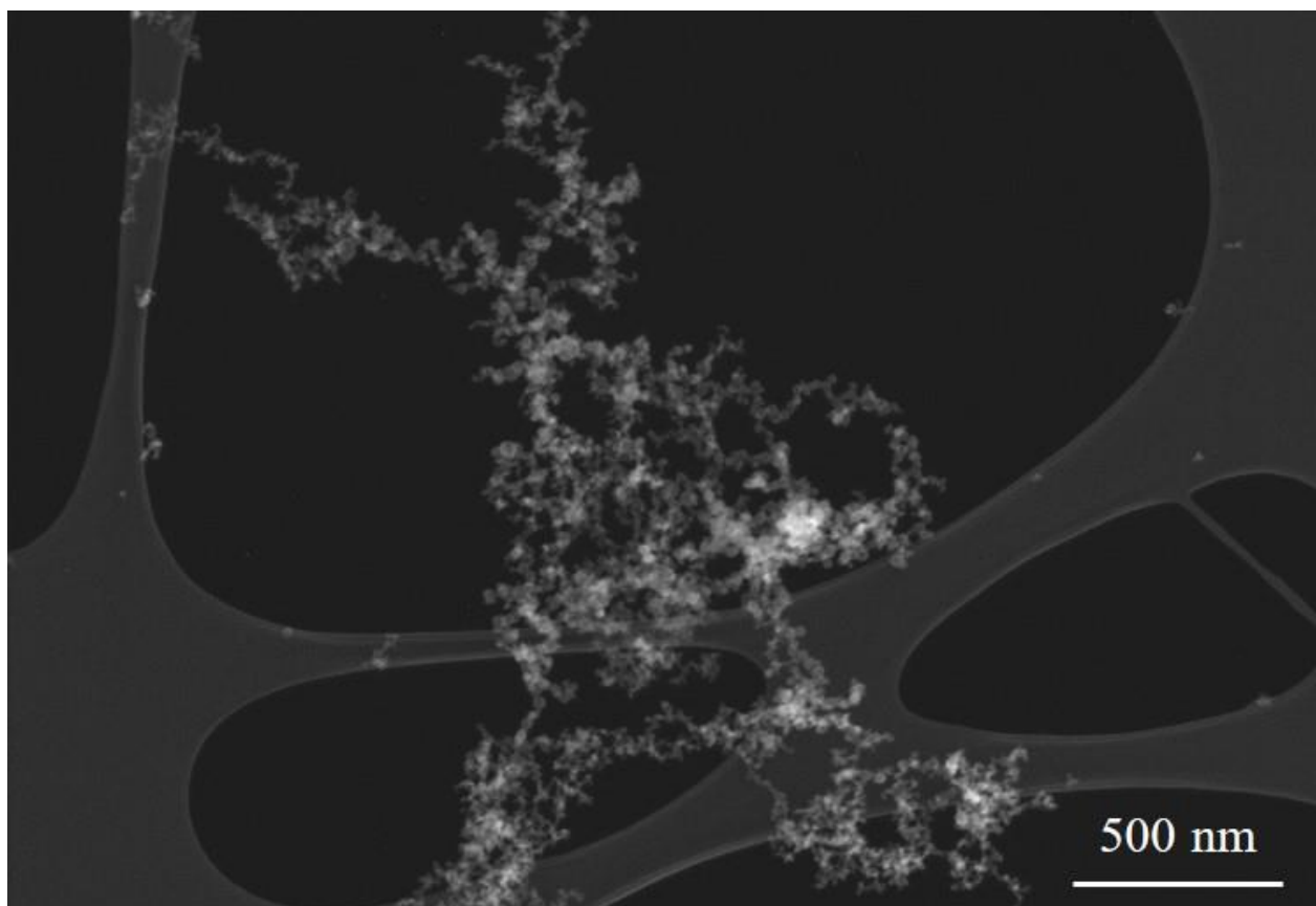
Figure 8.7 Secondary electron image of agglomerates/aggregates formed through laser cutting 6 mm stainless steel plates
