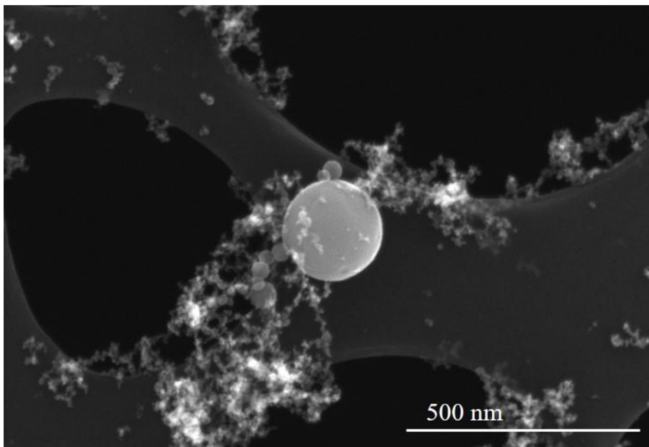
Figure 8.9 Secondary electron image of a large spherical particle ( d_g > 215 nm) found amongst steel agglomerates/ aggregates with various number of particles.
