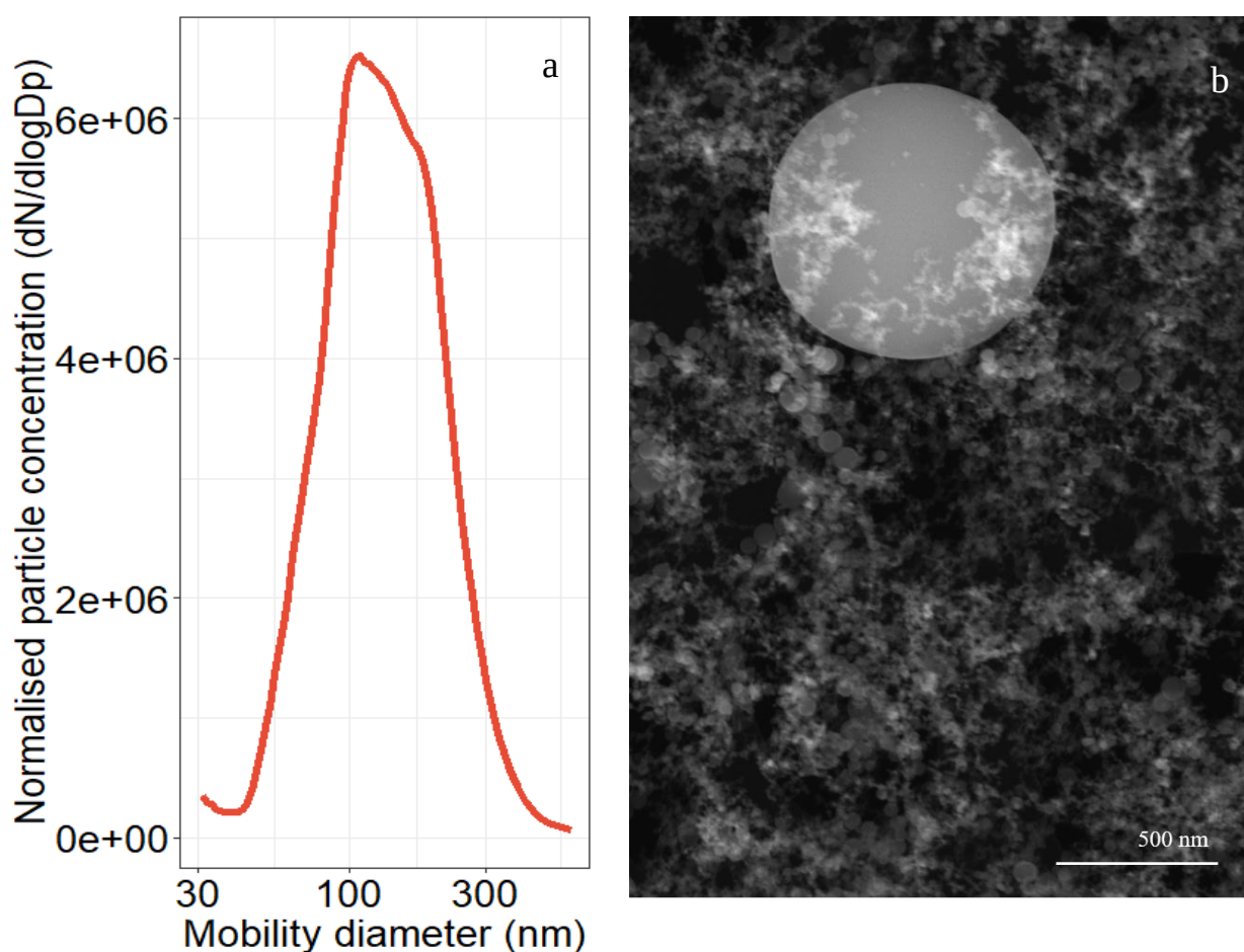
Figure 8.3 Average concentrations of particles from laser cutting a titanium-based plate by CO 2 -laser, as a function of d_{mob} (a), with corresponding secondary electron image of typical titanium-rich particles (b).
