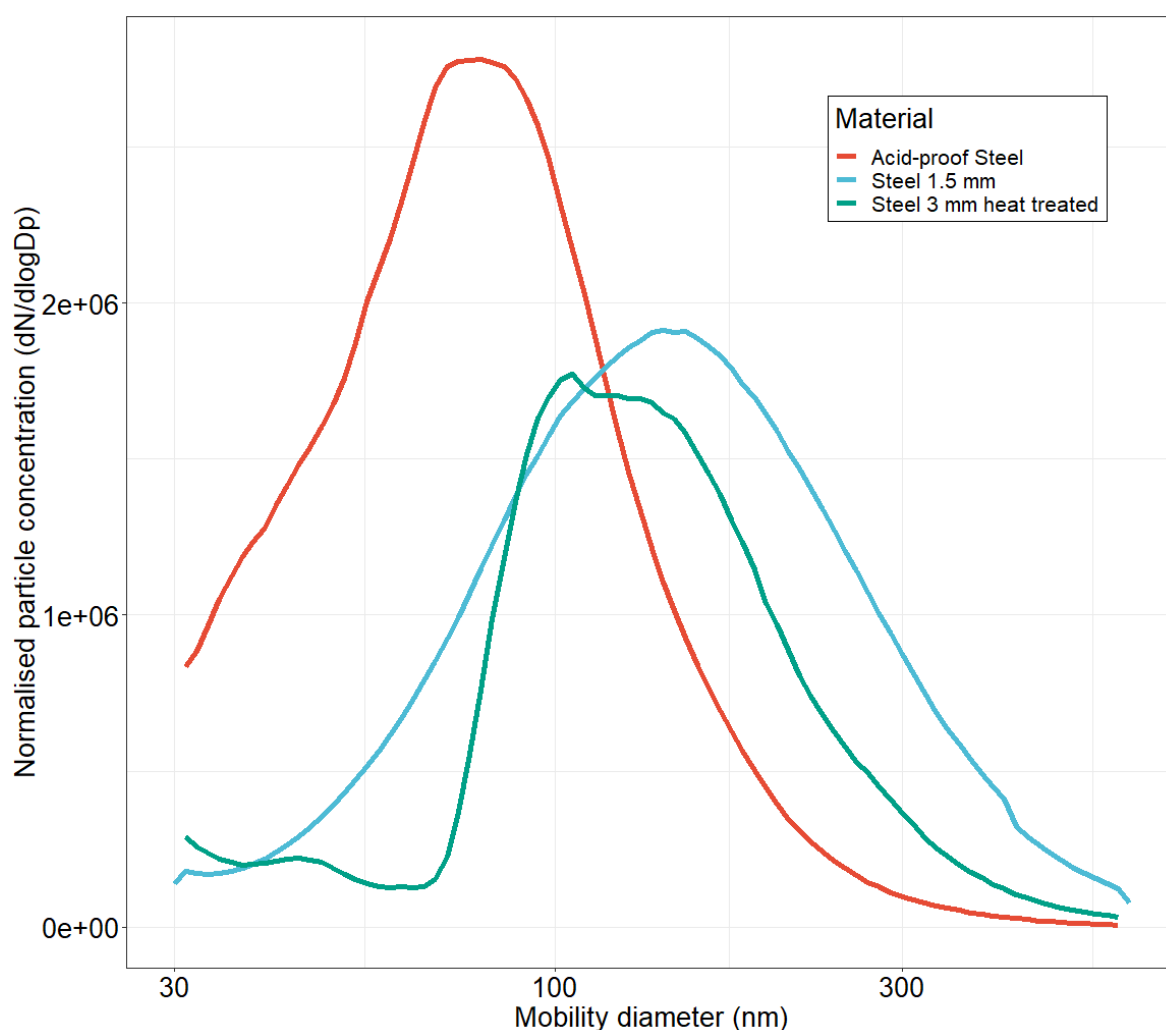
Figure 8.6 Average concentrations of particles from laser cutting selected steel plates by CO 2 -laser, as a function of d_{mob} .
