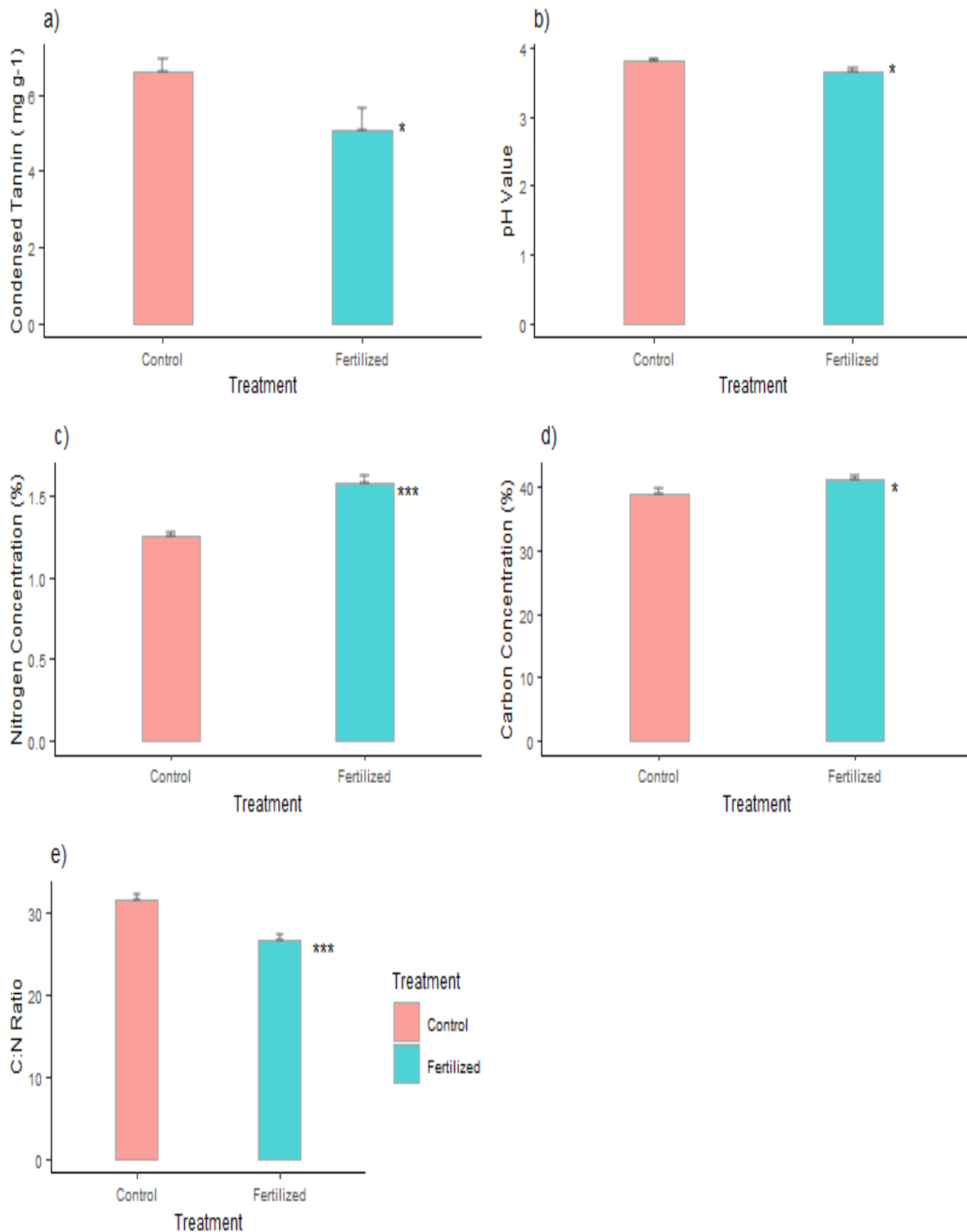
Figure 3: Mean values of response variables of soil with standard error (a) condensed Tannin Concentration, (b) pH value, (c) Nitrogen Concentration, (d) Carbon Concentration, (e) C: N Ratio (carbon to nitrogen ratio), for the two treatments. The mean value was calculated by dividing the total sum of the values by the number of plots, including subplots (n=50 for each treatment). Significant p-values for each response are shown by the asteroid ('*' and '***') beside the respective column.
