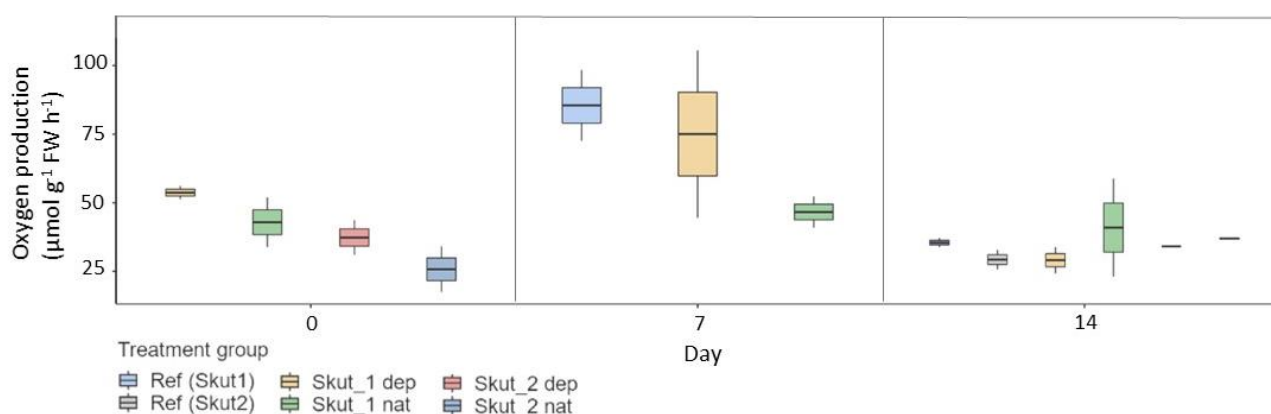
Figure 22: Oxygen production at 0-14 days into the field exposure study, for deployed (dep) and native (nat) moss Fontinalis antipyretica in Skuterud stream site 1 (Skut_1) and 2 (Skut_2), and moss tissue deployed into reference stream from Skut 1 (Ref (Skut 1)) and 2 (Ref (Skut 2)). No statistical significance could be calculated as n=2 .
