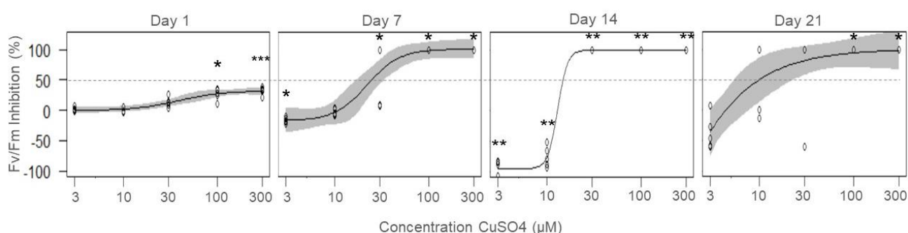
Figure 10: Inhibition of maximal PS II efficiency (Fv/Fm) in Fontinalis antipyretica after 1-21 days of exposure to CuSO 4 . Asterisks marks statistically significant difference to control (* p<0.05, ** p<0.01, *** p<0.001). Broken line marks the concentration causing 50 % inhibition.
