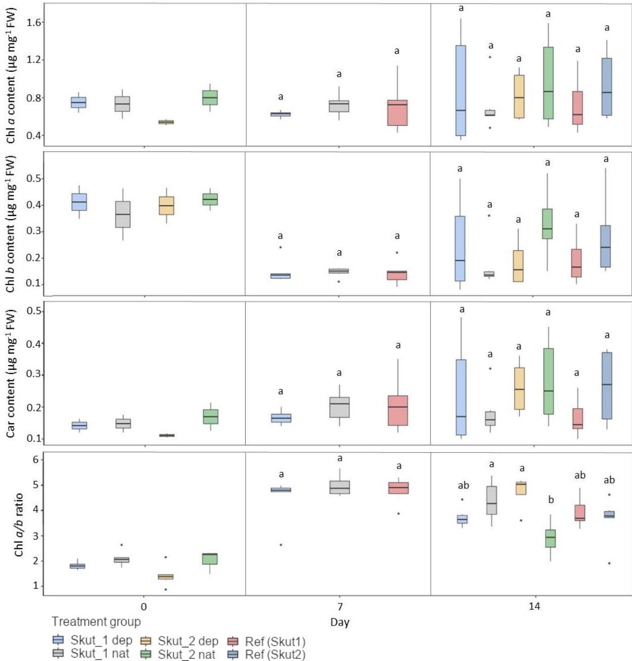
Figure 21: Concentration of pigments chlorophyll (Chl) a, Chl b and carotenoids (Car), and Chl a/b ratio at 0-14 days into the field exposure study, for deployed (dep) and native (nat) moss Fontinalis antipyretica in Skuterud stream site 1 (Skut_1) and 2 (Skut_2), and moss tissue deployed into reference stream from Skut 1 (Ref (Skut 1)) and 2 (Ref (Skut 2)). Significant difference ( p < 0.05 ) is encoded by letters (no statistical significance could be calculated at day 0 where n=2 ).
