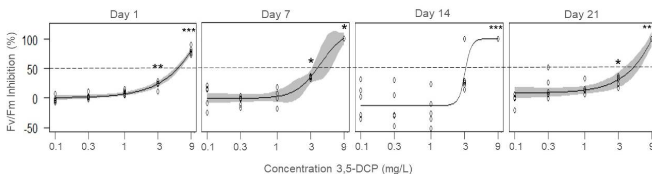
Figure 15: Inhibition of maximal PSII efficiency (Fv/Fm) in Fontinalis antipyretica after 1-21 days of exposure to 3,5-dichlorophenol (3,5-DCP). Asterisks marks statistically significant difference to control (* p < 0.05 , ** p < 0.01 , *** p < 0.001 ). Broken line marks the concentration causing 50 % inhibition.
