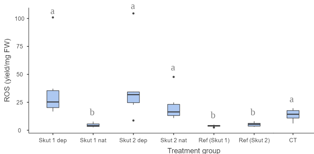
Figure 24: ROS yield for deployed (dep) and native (nat) moss Fontinalis antipyretica in Skuterud stream site 1 (Skut_1) and 2 (Skut_2), and moss deployed into reference stream from Skut 1 (Ref (Skut 1)) and 2 (Ref (Skut 2)) after 14 days exposure. CT is F. antipyretica grown at the lab in medium during the exposure period. Significant difference ( p < 0.05 ) is encoded by letters.
