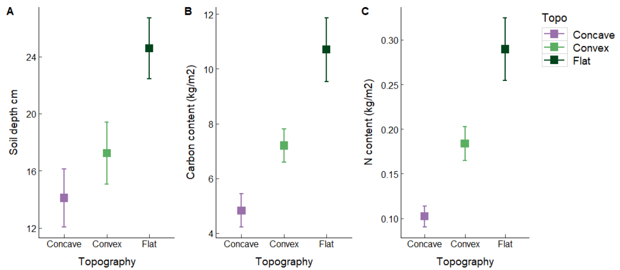
Figure A10: A) Mean \pm SE soil depth in relation to topography. B) Mean \pm SE carbon content in relation to topography. C) Mean \pm SE nitrogen content in relation to topography.
