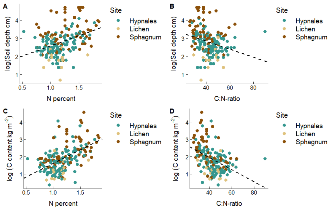
Figure 4: Relationships between A) soil depth and nitrogen percent, \beta=1.1165 , p=5.99e-08 , B) soil depth and C:N-ratio, \beta= -0.02184 , p= 2e-16 , C) soil carbon content and nitrogen percent, \beta=1.57140 , p= 1.27e-14 , D) soil carbon content and C:N-ratio, \beta=-0.035169 , p=1.71e-09 .
