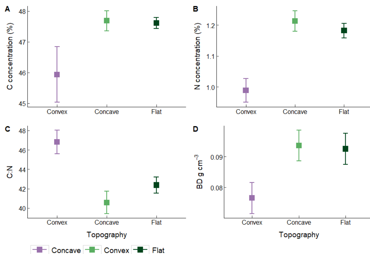
Figure 12: A) Mean \pm SE carbon concentration in the different topography classes. B) Mean \pm SE nitrogen concentration by topography type. C) Mean \pm SE C:N-ratio by topography type. D) Mean \pm SE bulk density by topography type.
