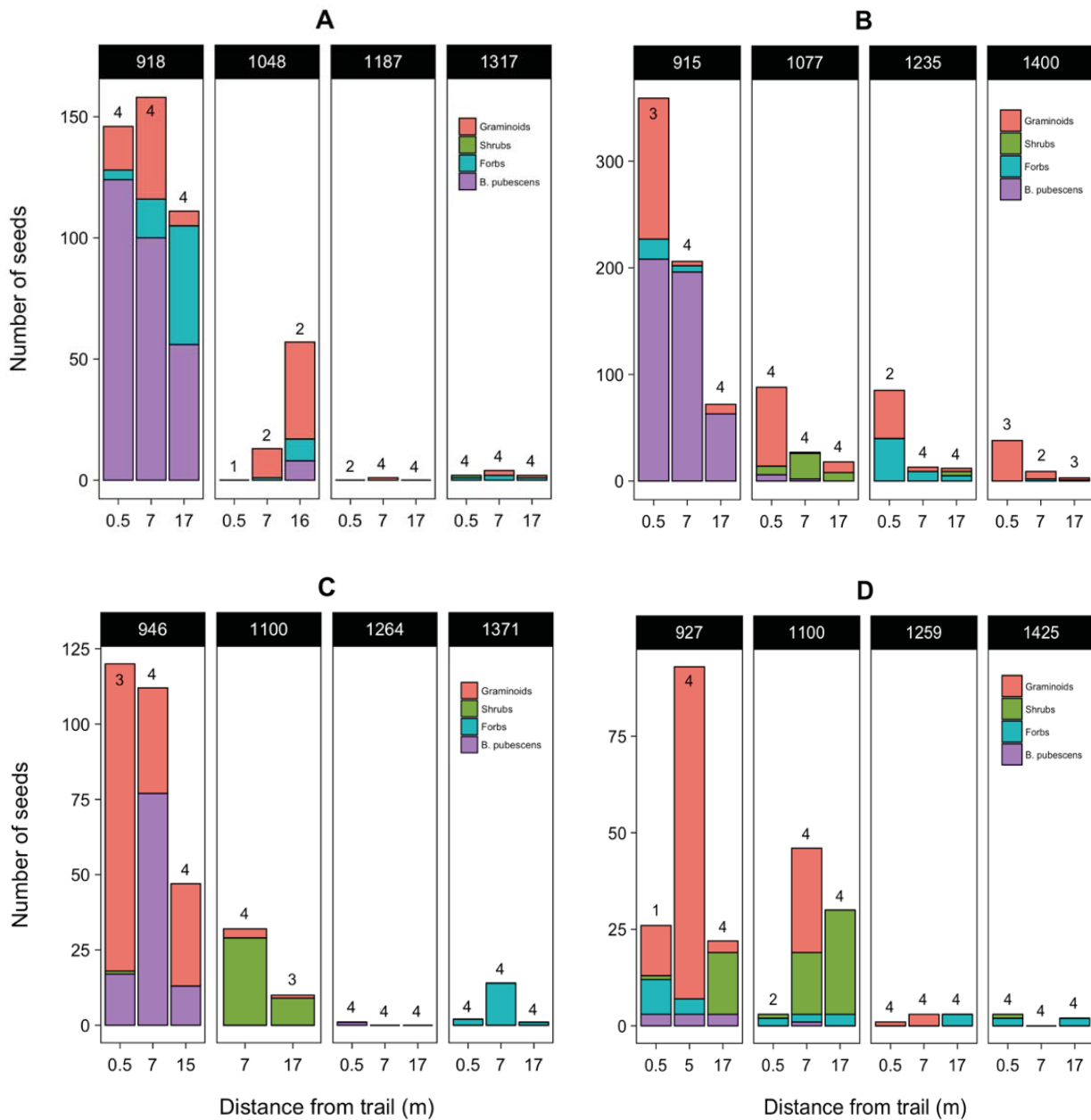
Figure 5. Raw number of seeds collected in seed traps. Note that not all seed traps were recovered/usable: data for each distance at each elevation is sourced from 1-4 traps (numbers in/above histogram bars). Numbers at top of sections denote transect elevations in metres. Letters in bold denote trail IDs.
