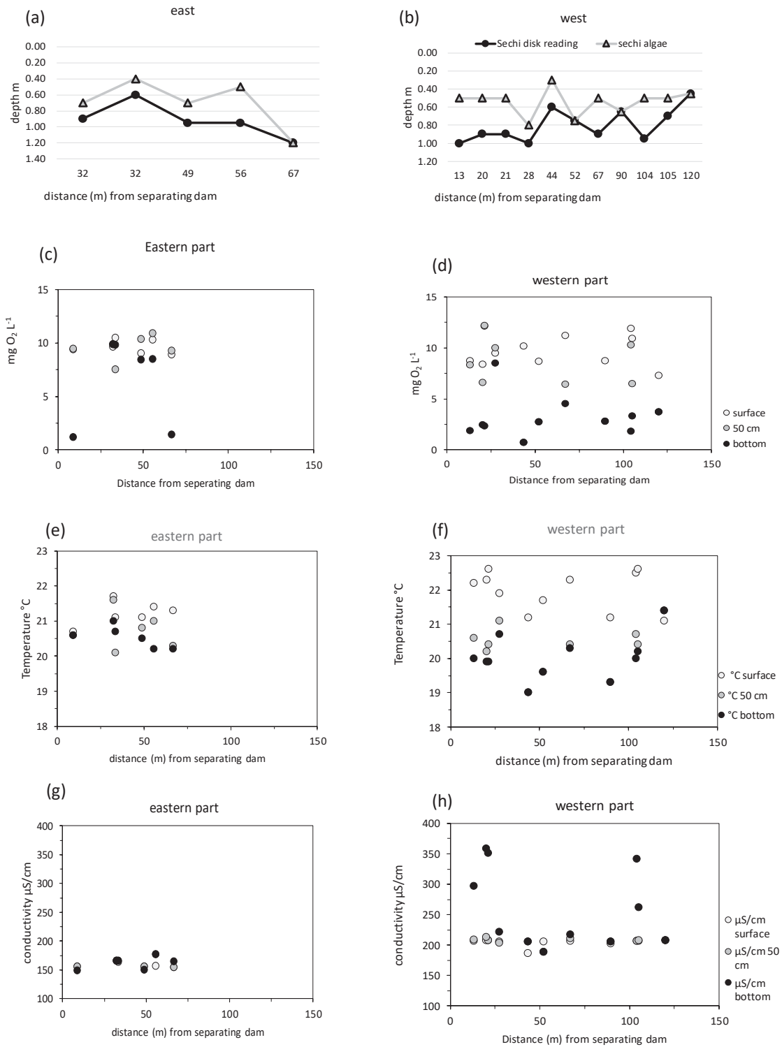
figure 2 data from transects sampled August 9 th . presented with sampling distance from a line that separates the the lake in two parts. a and b - Secchi-disk reading showing depth and top of filamentous algae in the two parts of the lake. c and d - concentration of dissolved oxygen \text{mg O}_2 \text{ L}^{-1} . Measured at surface, 50 cm depth and at the bottom. e and f -temperature measured at surface, 50 cm depth and at the bottom. g and h - conductivity \mu\text{S/cm} measured at surface, 50 cm depth and at the bottom.
