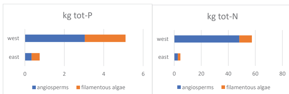
Figure 8 estimated total amount of tot-P and tot-N in macrophytes.
