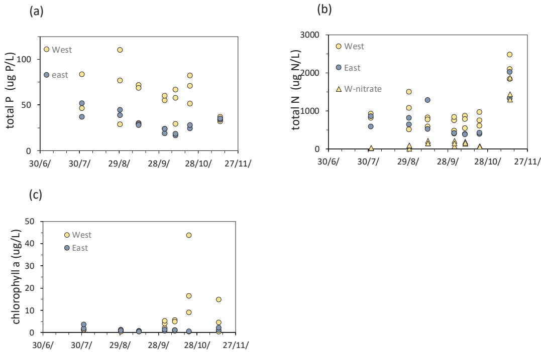
fig 3 a - concentration of total phosphorus \mu\text{g/L} . b - concentration of total nitrogen for both parts of the lake and nitrate from the western part \mu\text{g/L} . c - concentration \mu\text{g/L} of chlorophyll-a
