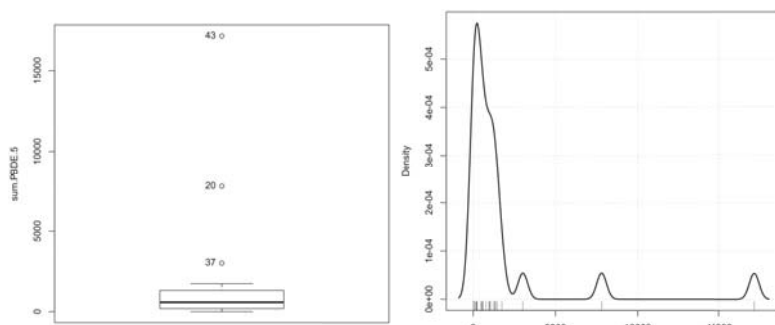
Figure B.2.1.4: Box- (left) and density (right) plots for the indicator PBDEs (congener number 47, 99, 100, 153, and 154). The numbers indicated: 43, 20, and 37 are: 53 (Aremark), 30 (Øvrevatn), and 47 (Utboja).
