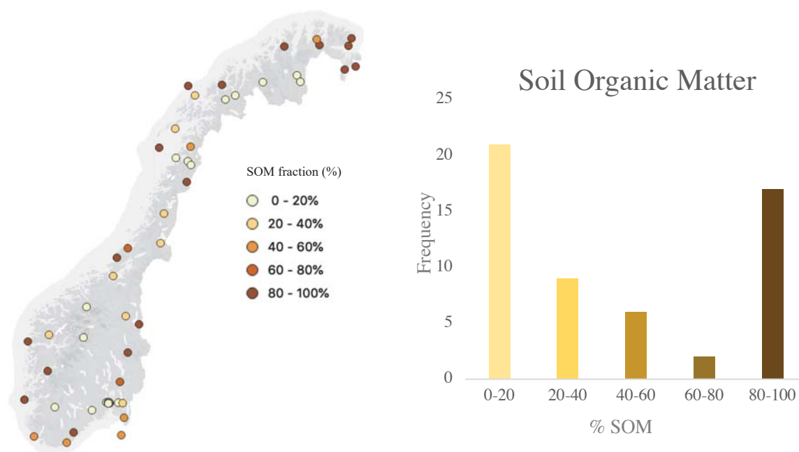
Figure 17: Distribution of SOM content for all soil samples included in this study, where x-axis is % SOM content intervals, and y-axis is the soil sample frequency within the intervals. The majority of the soil samples with 0-20% SOM were from the Oslo area urban soils. The number of samples with 80-100% SOM make up about 30% of all samples.
