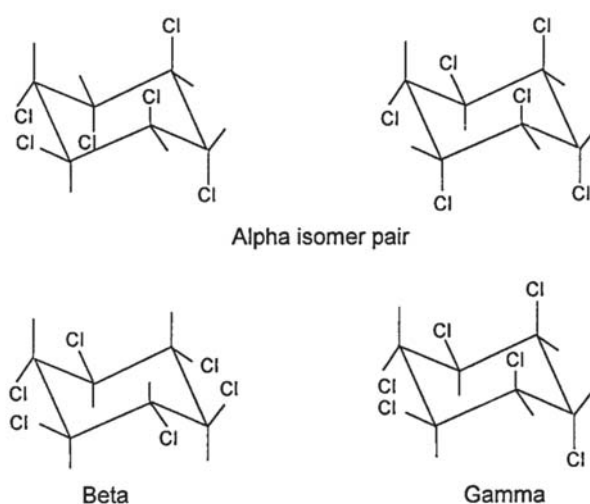
Figure 3: Structures of HCH-isomers, with two \alpha -enantiomers. These structures show the chlorine atoms spatial placement (Willett et al. 1998).
