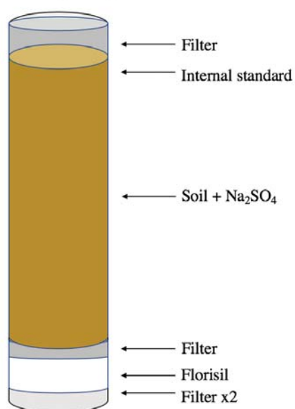
Figure A.2.1.1: ASE cell packing illustration.
