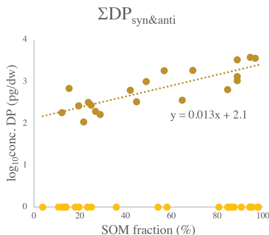
Figure 24: The relationship of \Sigma DP_{\text{syn\&anti}} with SOM content. The orange dots represent the values <MDL, where there is a nearly equal amount at low and high SOM content. The few samples <MDL observed at mid-SOM content could be related to the few samples with this SOM content (Figure 17). The strength of linear relationship was found to be r=0.8 and p<0.001 .
