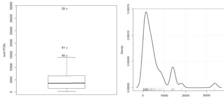
Figure B.2.1.1: Box- (left) and density (right) plots for PCBs. The numbers indicated: 25, 41, and 45, are: 35 (Aglen), 51 (Hvittingfoss), and 55 (Hurdal), respectively.
