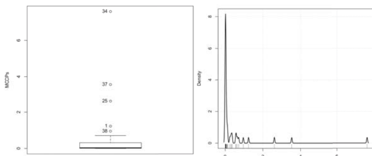
Figure B.2.1.7: Box- (left) and density (right) plots for MCCPs. The numbers indicated: 34, 37, and 25 are: 44 (Furumset), 47 (Utboja), and 35 (Aglen).
