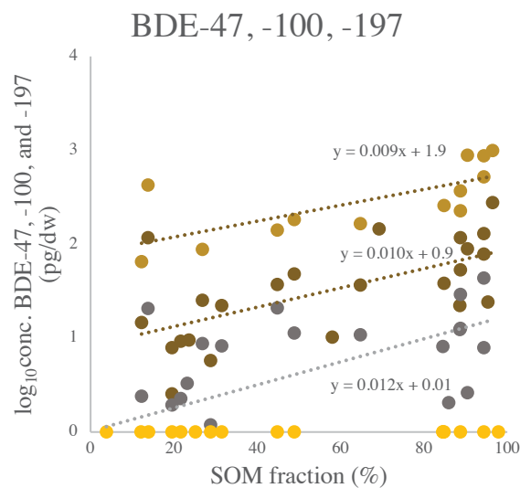
Figure 21: The relationship of selected indicator PBDE-congeners: from top to bottom dots and line: BDE-47, -100, and -197. The orange dots represent the values <\text{MDL} , where there is a higher frequency of these samples at lower SOM content. The strength of linear relationship through correlation test was found to be r\sim 0.6 ( p<0.05 ) for all congeners assessed. This figure also show that the concentration of PBDE-congeners decreases from BDE-47 to -197.
