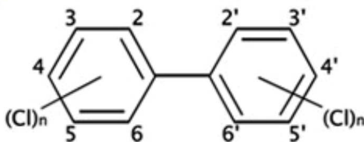
Figure 1: General PCB structure. The numbers indicates possible chlorine atom positions on each carbon atoms in the benzene rings (Lein 2017).
