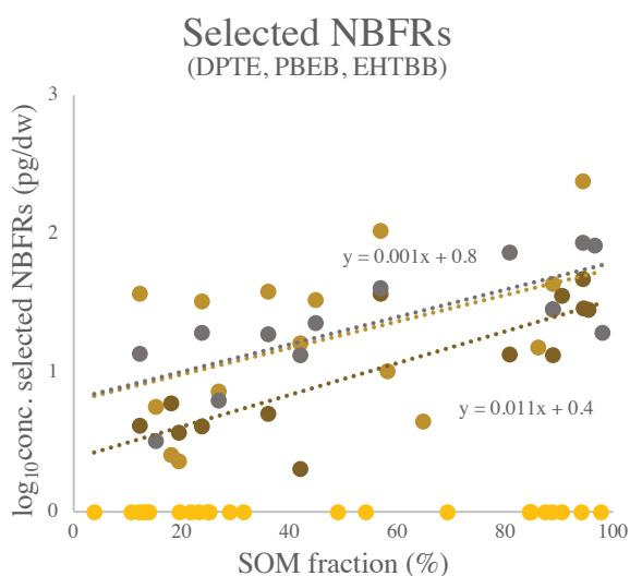
Figure 22: The relationship of selected NBFRs: from top to bottom dots and line: DPTE, EHTBB, and PBEB. The orange dots represent the values <\text{MDL} , where there is a slightly higher frequency of these samples at lower SOM content. The strength of linear relationship through correlation test was found to be 0.3 ( p<0.05 ).
