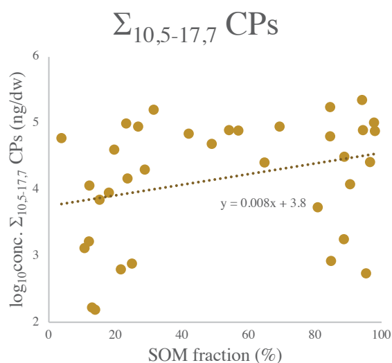
Figure 23: The relationship of \Sigma_{10,5-17,7}\text{CPs} with SOM content. The strength of linear relationship was found to be significant for SCCPs separately ( r=0.3 , p<0.05 ), but not for MCCPs ( r=0.2 and p>0.05 ).
