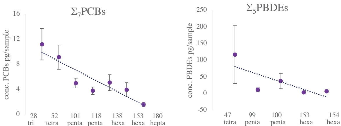
Figure 14: The distribution of \Sigma_7 PCB (left) and \Sigma_5 PBDEs (right) in blank samples ( n=8 ), where x-axis is PCB/PBDE-congeners with increased halogenation degree (tri-hepta), and y-axis is mean concentration in pg/sample with standard deviation.
