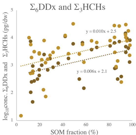
Figure 20: The relationship of \Sigma_6\text{DDx} (upper dots and line) and \Sigma_3\text{HCHs} (lower dots and line) with SOM content in n=42 and 40 soil samples, respectively. The strength of linear relationship through correlation test was found to be r=0.5 and 0.3 ( p<0.05 ), respectively.
