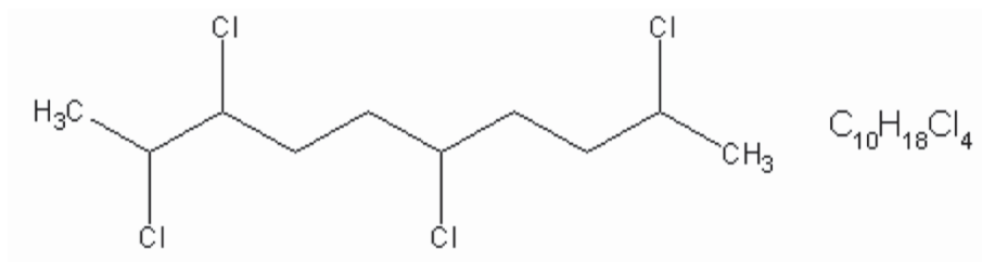
Figure 7: Chemical structure for the SCCP \text{C}_{10}\text{H}_{18}\text{Cl}_4 (UNEP 2016). For longer chains, the number of carbon atoms on the chain will increase, and for higher chlorination, the number of chlorine atoms on the chain will increase. Spatial position and number of chlorine atoms, and the length of the carbon chain, gives different congeners of CPs.
