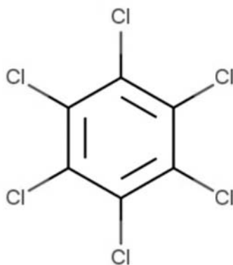
Figure 4: Chemical structure of HCB (ECHA 2019). The molecular formula for HCB is C_6Cl_6 .
