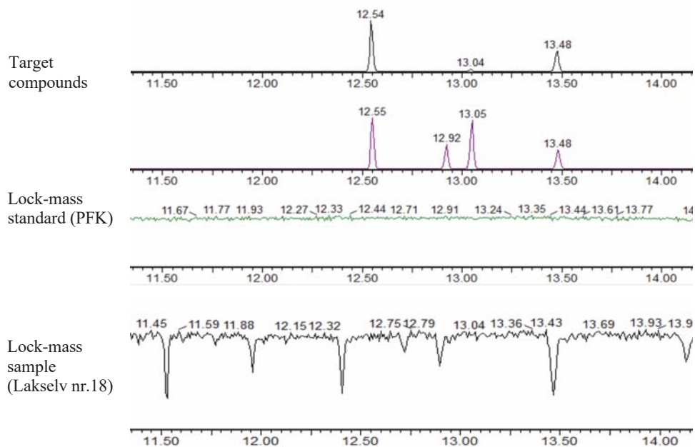
Figure 15: Example of drops in the lock-mass signal. This figure shows the constant, stable signal from the lock-mass standard (green), and the repetitive drops in the lock-mass signal from sample 18 Lakselv. These “pulses” of drops are caused by alkanes from the SOM. However, none of the drops are found at the elution times for the target compounds, and the quantification is consequently not affected in this sample.
