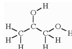
Figure 2.7 – Molecular structure of Propylene Glycol (moleculardimensions.com)
