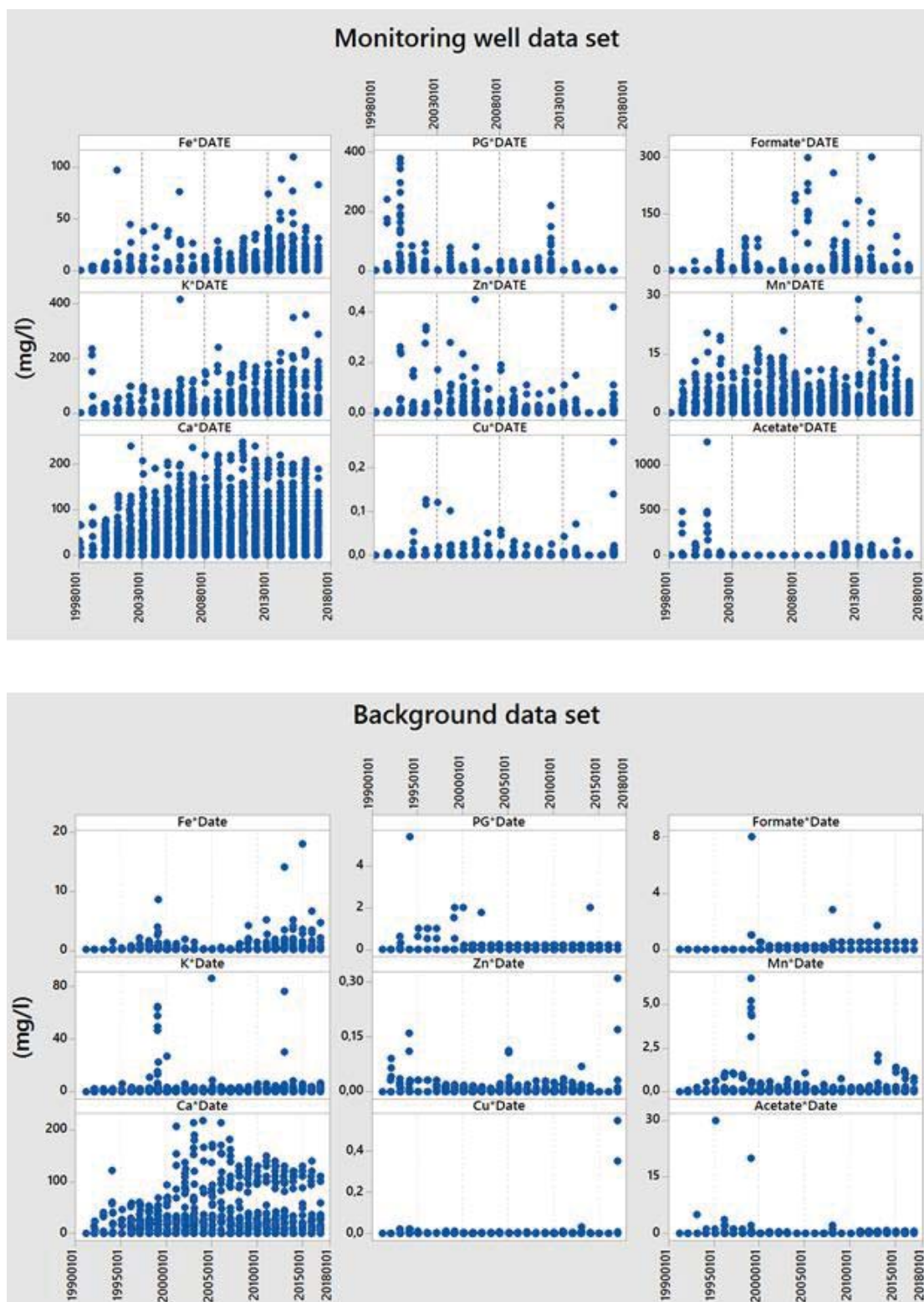
Figure 4.3 – Concentration of various chemical parameters in two wells data sets. Monitoring well show high values than background data set in most parameters.
