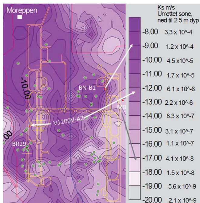
Figure 4.9 – Hydraulic conductivity distribution in upper 2.5m of unsaturated zone over OSL, (modified from French, Helen K. et al. (2000)).
