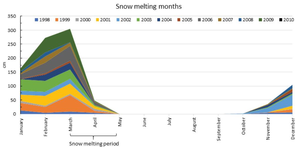
Figure 4.7 – Snow accumulating and snow melting months.
