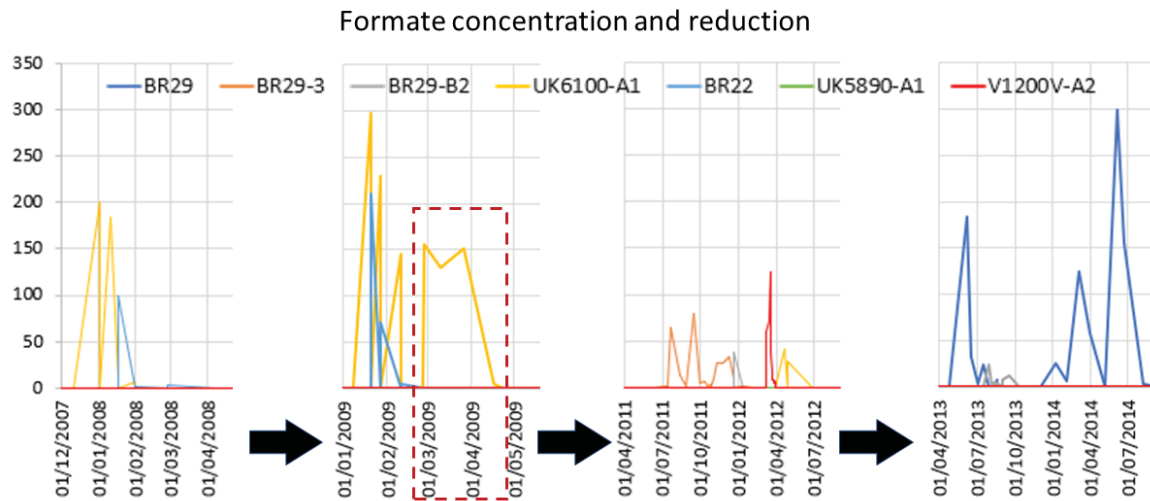
Figure 4.15 – History of formate concentration (mg/l) in affected wells. Red rectangle indicates addition of formate during March and April 2009.
