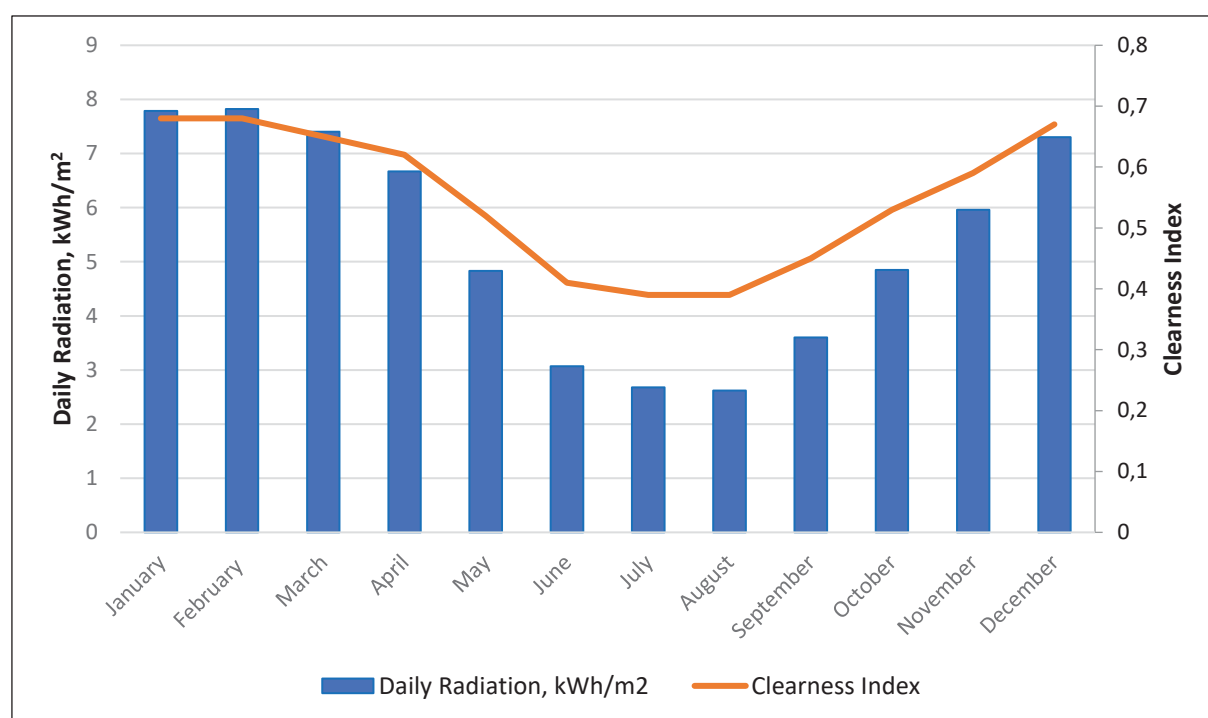
Figure 3.1: Daily average monthly solar radiation (kWh/m2) and clearness index in Amatgyi Khone village
