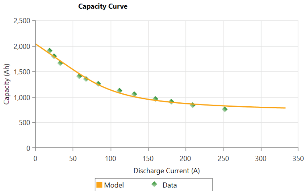
Figure 4.5: Capacity curve of Surrette 4KS25P, 4V battery
