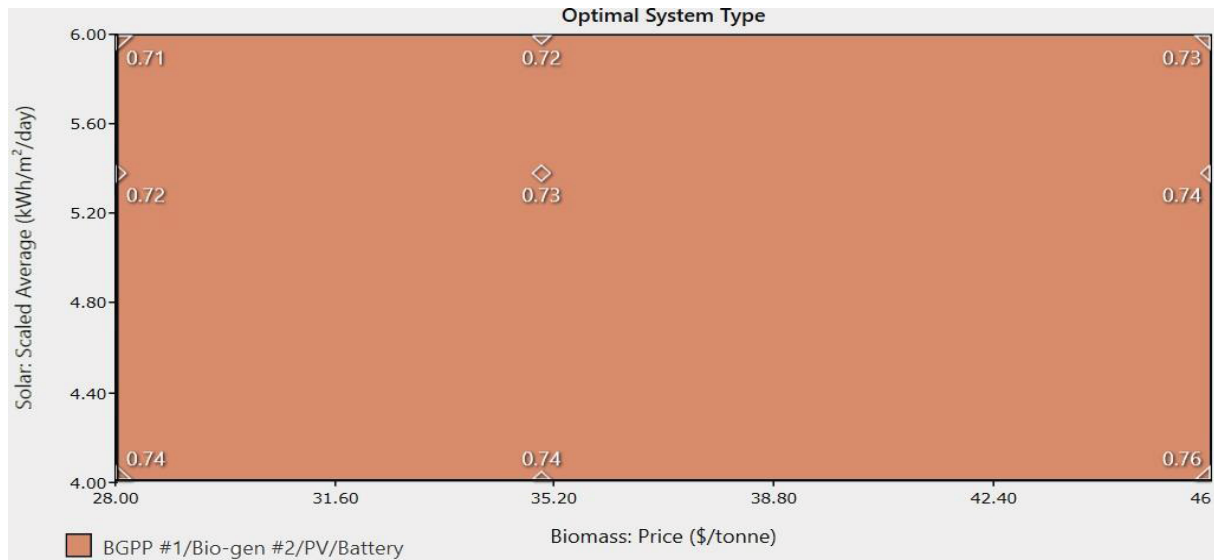
Figure 6.7: Illustration of optimal system type where values of COE are shown due to variations of annual scaled solar radiation ( \text{kWh/m}^2/\text{day} .) and rice husk prices ( \$/\text{tonne} ).
