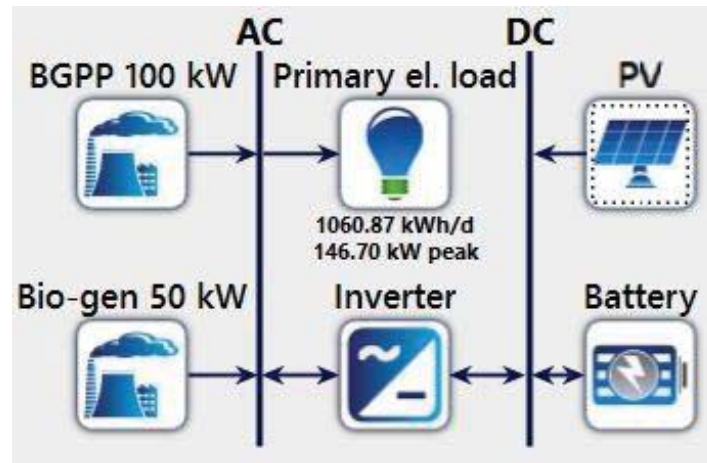
Figure 5.1: Selected HRES AC/DC bus coupling
