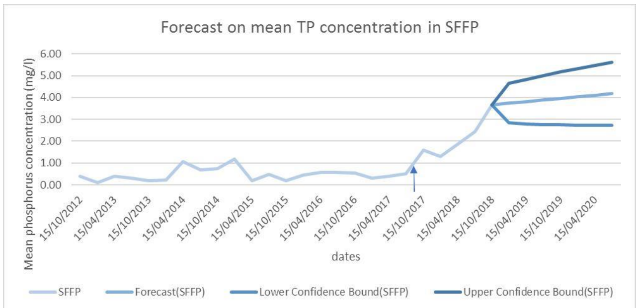
Fig 4.3: Forecast curve of when mean TP effluent concentration crosses the 1mg/l in the SFFP.
