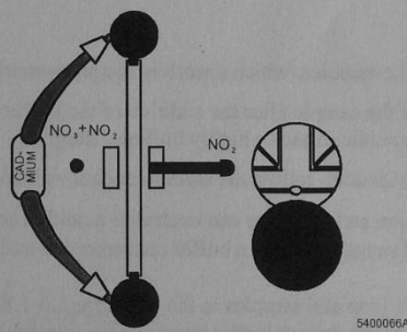
Figure 2. \text{NO}_2 position
