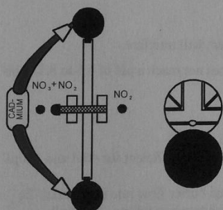
Figure 1. \text{NO}_2/\text{NO}_3 position
