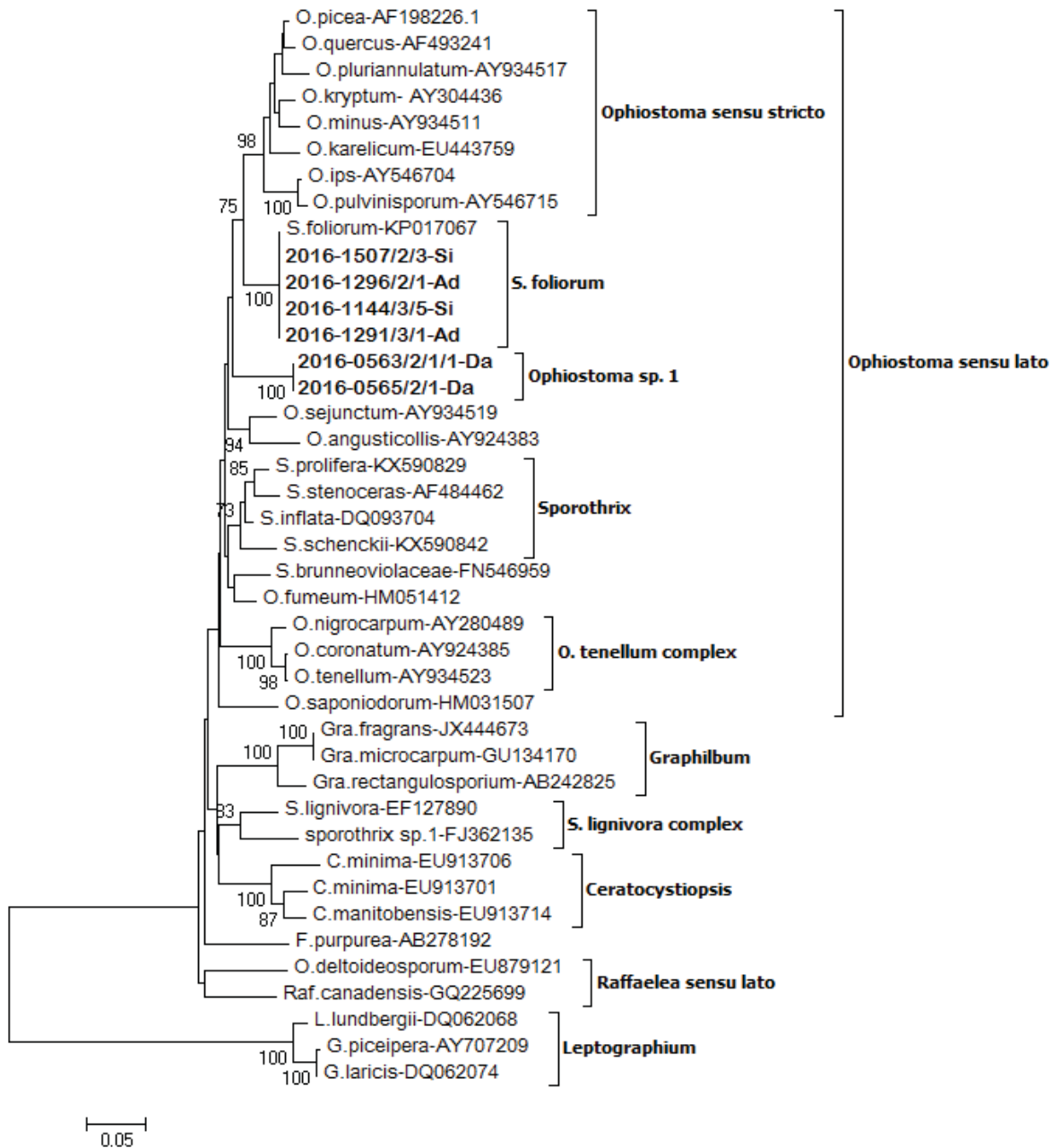
Figure 10. Phylogram based on ITS Sequences of the major clades within the Ophiostomatales . Bootstrap support values (1000 replicates) above 70% are indicated next to the branches. All positions containing gaps and missing data were eliminated. There were a total of 303 positions in the final dataset. Isolates sequenced in this study are printed in bold. Bar = number of base pair differences per site. The letters after the isolate numbers indicate: Ad, Anisandrus dispar ; Da, Dryocoetes alni ; Si, Scolytus intricatus .
