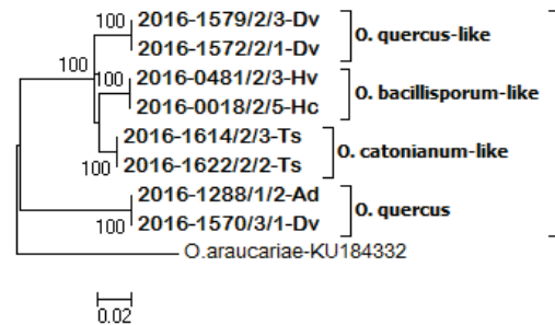
Figure 2. Phylogram based on (a) \beta -tubulin and (b) EF1- \alpha and (c) calmodulin sequences of species in the O. quercus group rooted to (a & b) O. novo ulmi or to (c) O. araucariae . Bootstrap support values (1000 replicates) above 70% are indicated next to the branches. All positions containing gaps and missing data were eliminated. There were a total of 249 positions in the \beta -tubulin dataset, 190 positions in the EF1 \alpha dataset and 539 positions in the calmodulin dataset. Isolates sequenced in this study are printed in bold. Bar= number of base differences per site. The letters after the isolate numbers indicate; Ad, Anisandrus dispar ; Dv, Dryocoetes villosus ; Hc, Hylesinus crenatus ; Hv, Hylesinus varius ; Si, Scolytus intricatus ; Sl, Scolytus laevis ; Sr, Scolytus ratzeburgi ; Td, Trypodendron domesticum ; Ts, Trypodendron signatum
