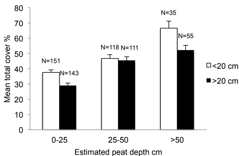
Figure 7: Mean total cover for the 613 logs studied at different estimated peat depths. White bars show logs with a mean diameter < 20 cm, while logs with a mean diameter > 20 cm are shown in black. SE and number of observations in each group shown on top of each bar.
