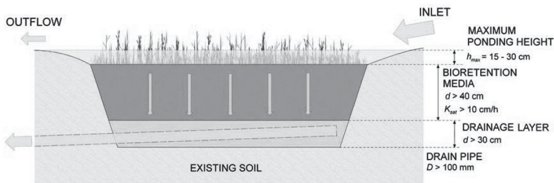
Figure 5. Principles of raingarden design (Paus & Braskerud, 2014).
