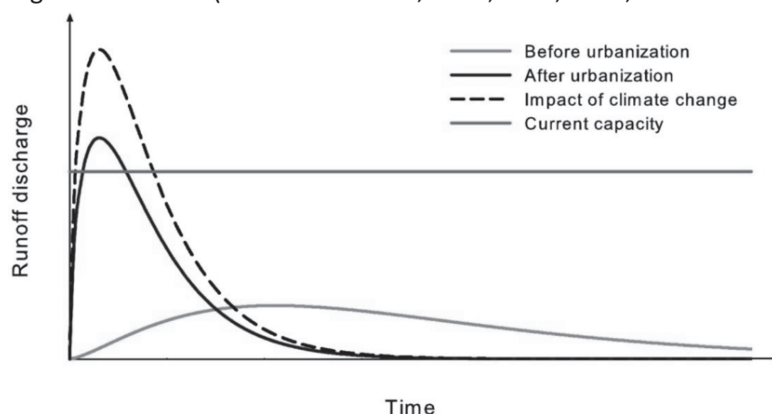
Figure 2. Effects of urbanization and expected outcomes of climate change on the runoff hydrographs (Paus, 2015).
