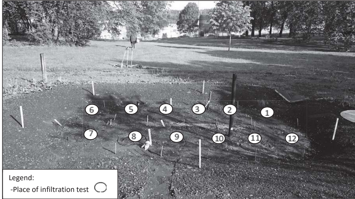
Figure 13. Places of infiltration test in the raingarden
