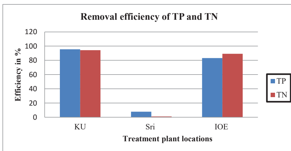
Figure 29: Removal efficiency of nutrients of each wetland
