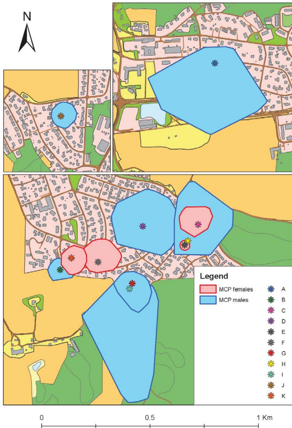
Figure 9. Individual total 99 % MCP for the 11 cats, separated into males (blue) and females (red). Asterisk marks the house belonging to the cat owner. The spatial positions of the home range and home of cat A and cat J are shown in figure 1.
