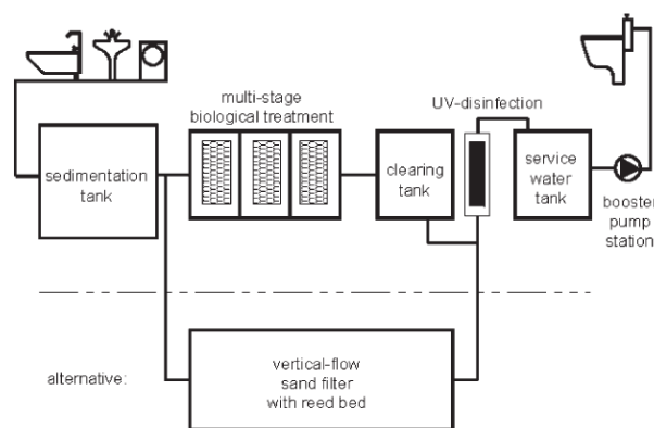
Figure 5, Recommended concept for greywater treatment from Nolde (2005). Note that a vertical flow sand filter reed bed (i.e. vertical constructed wetland) can replace a multi-stage biological treatment unit and cleaning tank.
