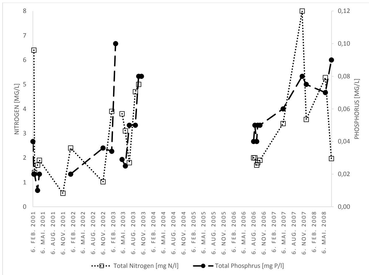
Figure 13, Data for effluent concentrations for the KL treatment system between 2001 and 2008.
