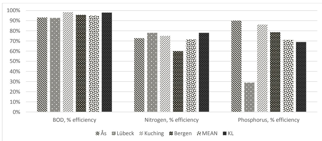
Figure 24, treatment efficiencies (%) for each of the cases Ås, Lübeck, Kuching and Bergen, as well as the the mean value of these systems. The 2014 KL average value is also included.
