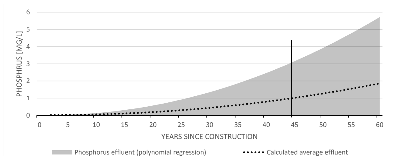
Figure 19, integral of the best fit (polynomial) regression (grey area), divided by number of years was calculated (dotted line). It was found that the average effluent would be 1 mg P/l after a lifetime of the filter of 45 years (black vertical line).
