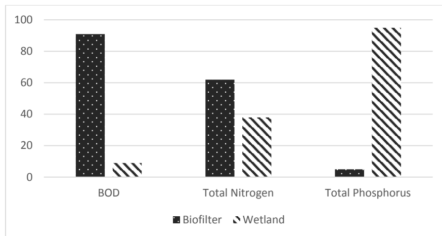
Figure 3, Relative treatment efficiency (%) for Biofilters compared to constructed wetlands. Graph based on numbers from Jenssen et al. (2006)
