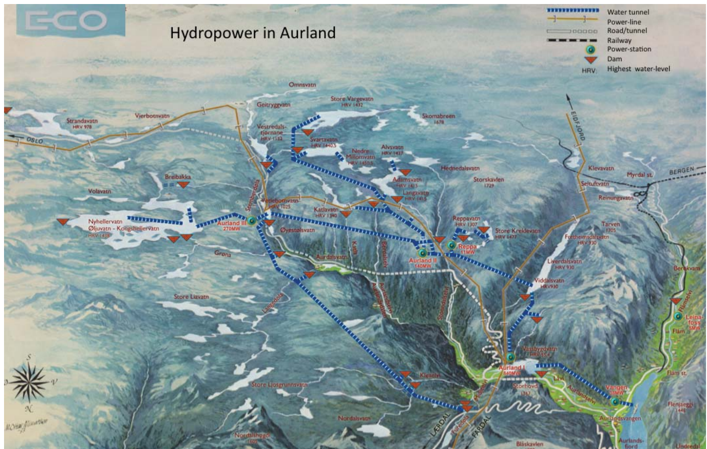
Figure 2 Map over the watershed and the regulation scheme in Aurland provided by E-CO Energy
