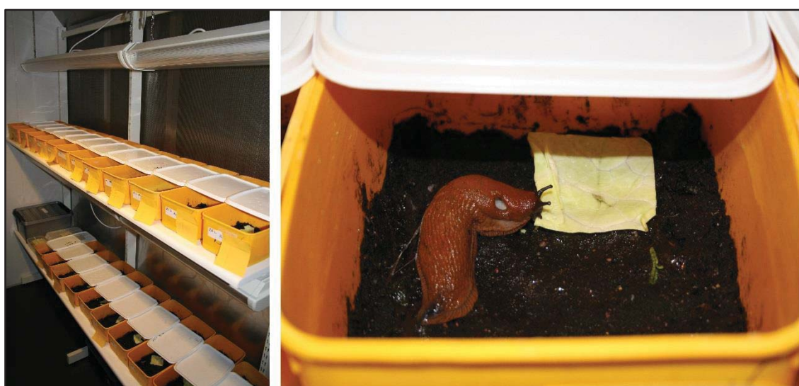
Figure 3: Left: The bioassay setup with 45 half covered plastic boxes. Right: An A. vulgaris in its arena, feeding on a cabbage square (4 x 4 cm).
