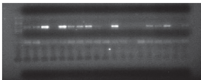
Figure 4: Image from the Bio-Rad Universal Hood II Gel Imager, showing the DNA ladder (on the left hand side) and the amplified 658 bp DNA fragments. Brightly coloured bands indicate successful extraction and PCR, and such samples were sequenced.
