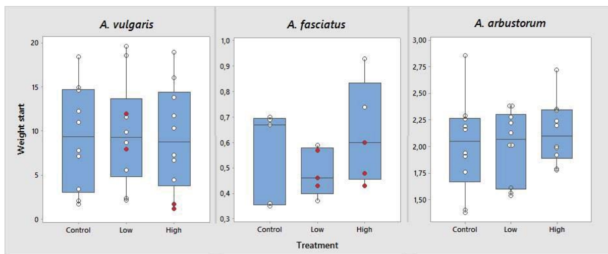
Figure 11: Box plots of start weight distribution (grams) of the gastropods used in the two bioassays (except the first batch A. fasciatus ). Boxes represent middle 50 % of weights, “whiskers” the upper and lower 25 %, and horizontal line indicates median. Individual specimens are indicated by dots, red dots being those that died.
