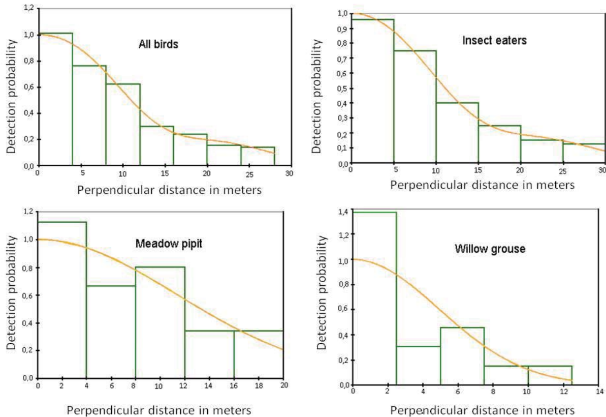
Figure 9: Distribution from transect line for the study groups all birds, insect eaters, meadow pipit and willow grouse and the best fit half-normal key function with a cosine series extension used as distance detection function.
