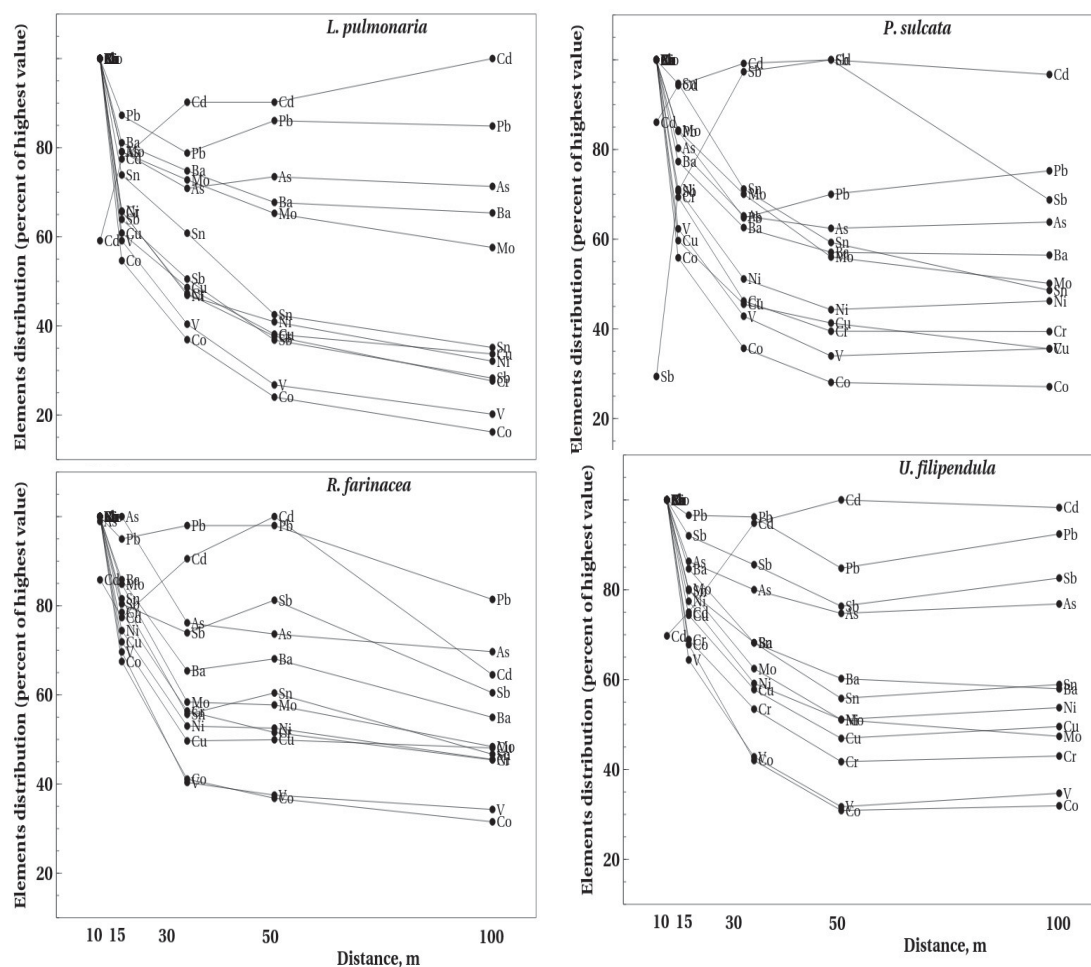
Figure 10. – Effect of distance (m) from the road on the trace elements distribution among the lichen species. Presented as percent (%) of the highest value
