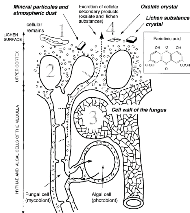
Figure 1. – Possible locations and uptake mechanisms of metals in the lichen thallus: (1) metal-rich particulate entrapment on the lichen surface and in intercellular spaces of fungal biont; (2) intracellular complexation to metallothioneins; (3) extracellular complexation to functional groups of fungal macromolecules from the cell walls; (4) extracellular complexation to organic acids, such as oxalate, or lichen substances, such as parietinic acid (adopted from Honegger 1991)
