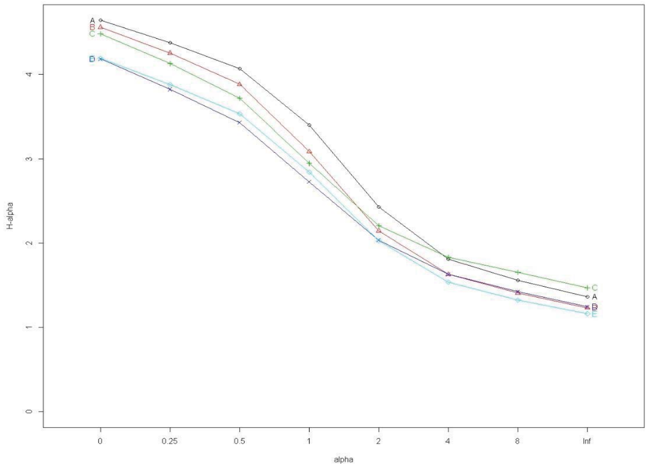
Figure 10 The Renyi diversity profile shows the difference in evenness, species richness and biodiversity among species between the different plots, based on aggregated data from 51 sites. The figure shows Renyi diversity profiles for each habitat. Steep curves indicate lower evenness among beetle species. The starting position on the left ( \alpha = 0 ) indicate that A, B and C has the largest beetle species richness, ranked in respective order. It is not possible to separate E and D. The antilog ( e^{H\text{-value}} ) for \alpha = 0 , shows the number of species richness. It is not possible to decide which site was the most diverse since the lines were crossing. Alpha = infinitive shows that the later forest edge habitat (C) had the least number of the most dominating species and the forest habitat a 100 m from the center of the power line habitat (E) had the largest number of dominating species. The forest habitat (D) and the early succession forest edge (B) have approximating equal numbers.
