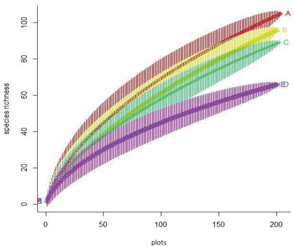
Figure 4 Species accumulation curves plotted for the five habitats. The x-axis shows the number of plots for collecting of beetles by sweep nets (see Figure 2). The y-axis show the cumulative numbers of species recorded. The habitat under the power-line (A) had the largest species richness and the lowest was in the forest habitat 100 m from the center of the power-line (E) and the forest habitat (D). The edge of the early succession habitat (B) had higher richness than the forest edge (C). The largest differences in species richness were found between the habitat in the center of the power-line had larger species richness, than the forested habitats (D and E). The vertical lines show the corresponding standard deviation.
