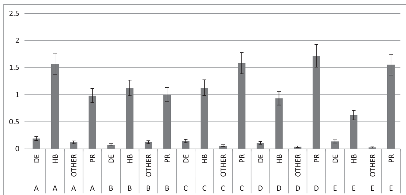
Figure 12 Estimated mean (±SE) number of individuals within different functional groups of beetles. Beetles were captured by sweep netting within 4m x 5m plots (see Figure 2) at 51 sites, in five different habitats: The center of the power-line habitat (A), the early succession edge habitat (B), forest edge habitat (C), forest habitat (D) and the forest habitat, a 100 m from the center of the power-line (E). PR = predators, HB = herbivores, DE = general detritivore and dead wood feeders and fungivores are grouped into the category 'OTHER'.
