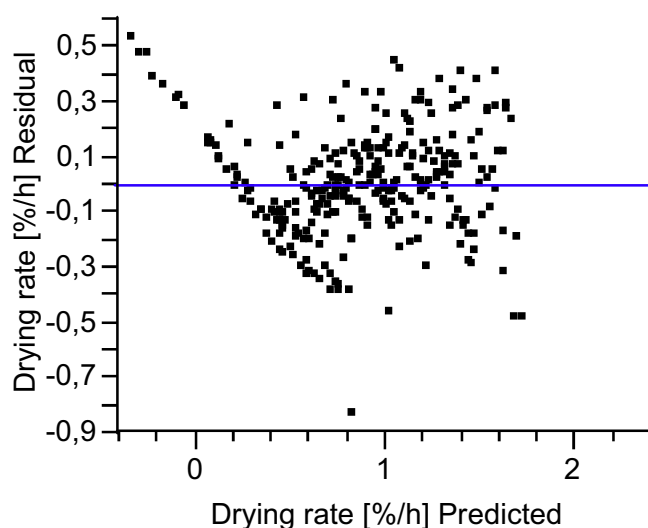
Figure 21. The residual plot for the model drying rate = f(\text{time, program, program*time, board number, initial moisture content}) .
