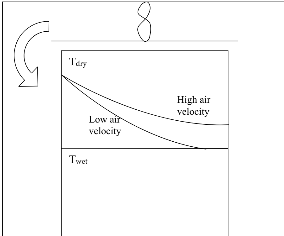
Figure 3. Dry and wet bulb temperature as it moves through a batch of moist lumber. At low air velocity air gets saturated before leaving the batch, which is not the case when the air velocity is high enough.
