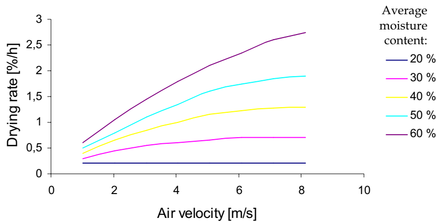
Figure 2. Effect of air velocity on the drying rate of sugar maple sapwood at a temperature of 54 °C (130 °F) and a relative humidity of 76 %. Based on the results from Torgeson (1951).
