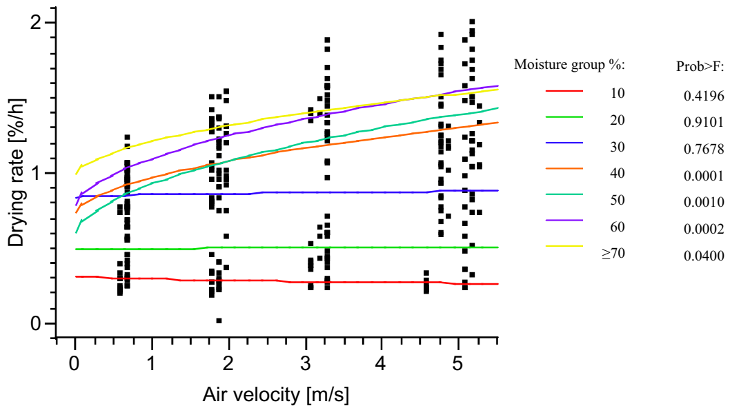
Figure 22. The drying rate at different air velocities for different moisture content with corresponding p-values to the regression fit of drying rate over \sqrt{(\text{air velocity})} . Drying rate is the average drying rate up to each measurement, air velocity is the average air velocity up to each measurement, and moisture content is rounded of to nearest 10 %.
