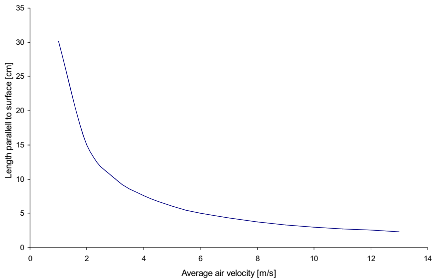
Figure 5. The levels of length parallel to the surface and the air velocity giving turbulent flow (reynolds number=20,000).
