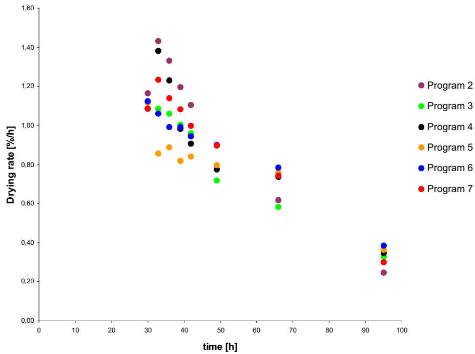
Figure 15. Average drying rate over time for the six programs.
