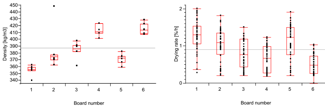
Figure 18. The drying rate and density for the six different boards.
