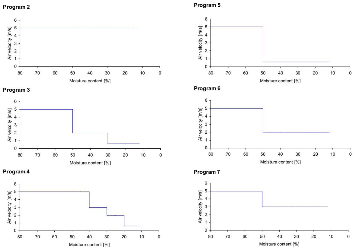
Figure 9. The reduction of air velocity for program 2-7. The moisture content is the expected moisture content according to TORKSIM.
