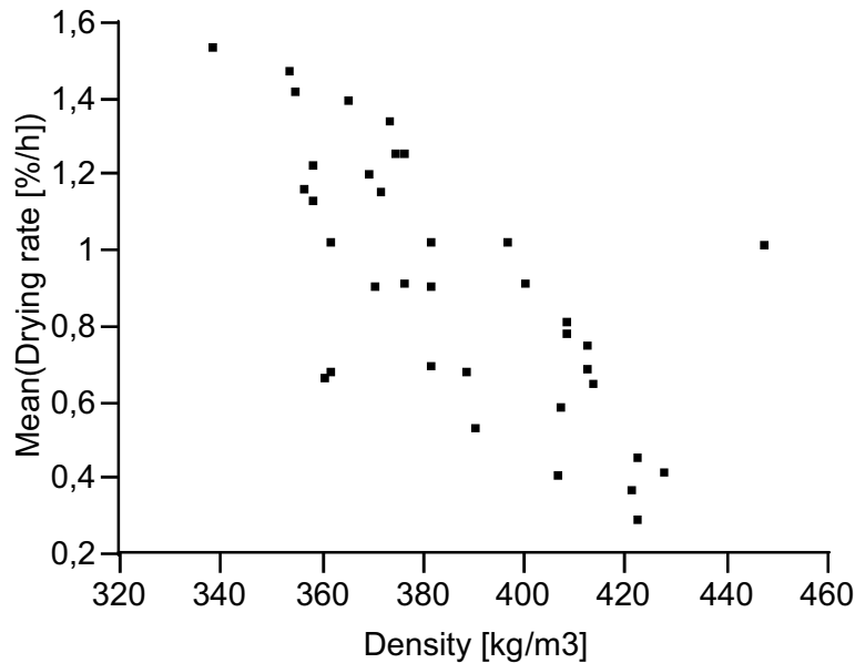
Figure 16. Average drying rate and density for each of the 36 samples.
