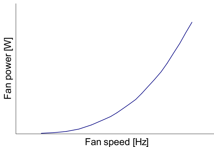
Figure 1. The relationship between fan speed and fan power (based on formula 1).
