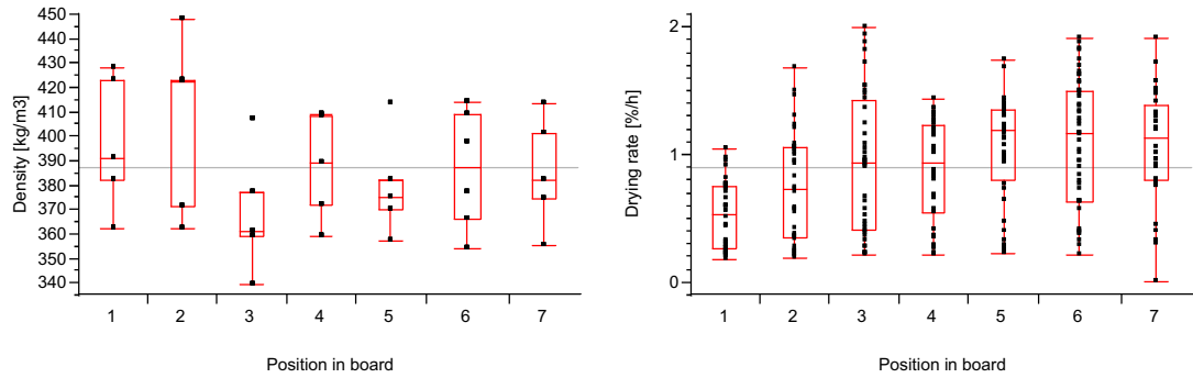
Figure 19. The drying rate and density for the seven positions in the boards.
