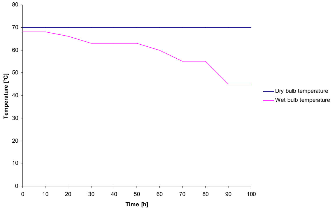
Figure 10. Dry bulb and wet bulb temperature in the experiment.
