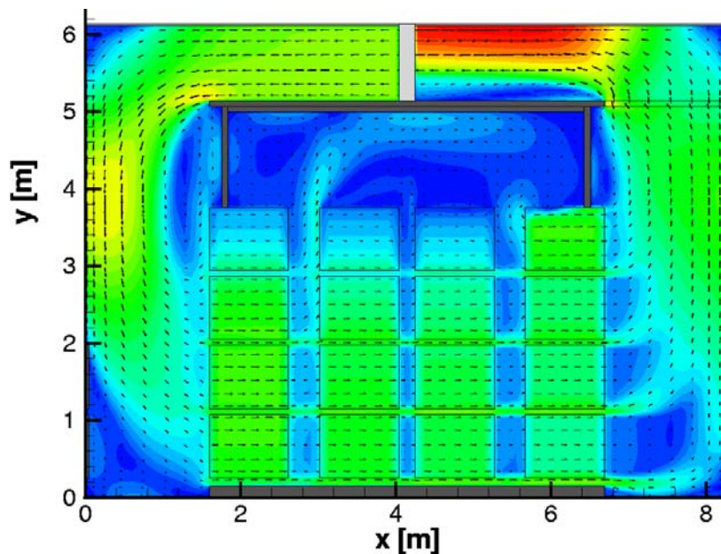
Figure 6. Airflow distribution in an industrial convection kiln showing velocities in the stack from 2 m/s (blue) to 5 m/s (red) (Riepen & Paarhuis 1999).
