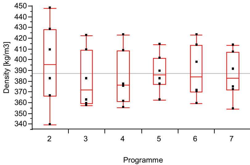
Figure 17. The density of the samples in the six programs.
