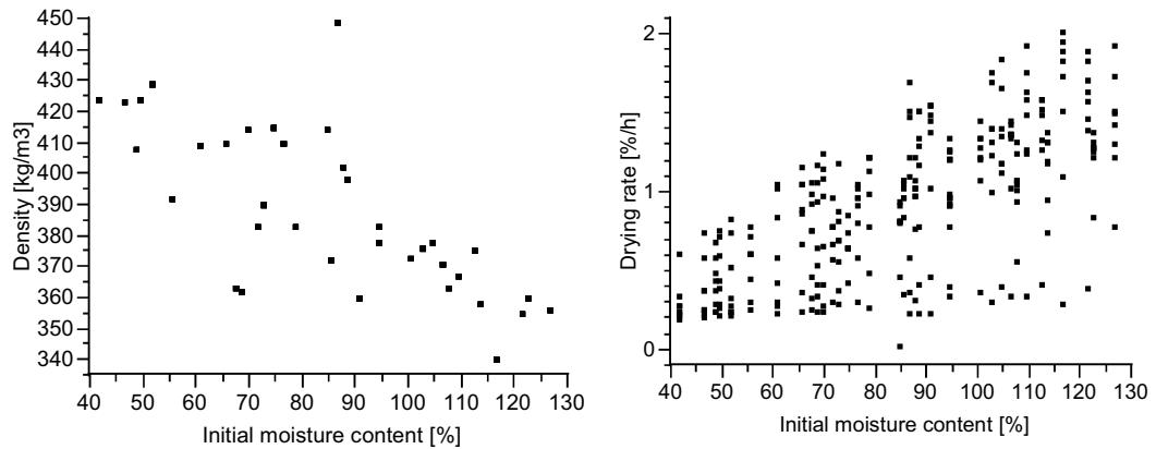
Figure 20. The drying rate and density for varying initial moisture content.
