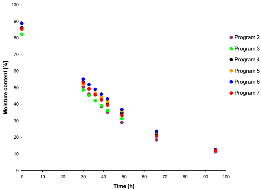
Figure 13. Average moisture content over time for the six programs.
