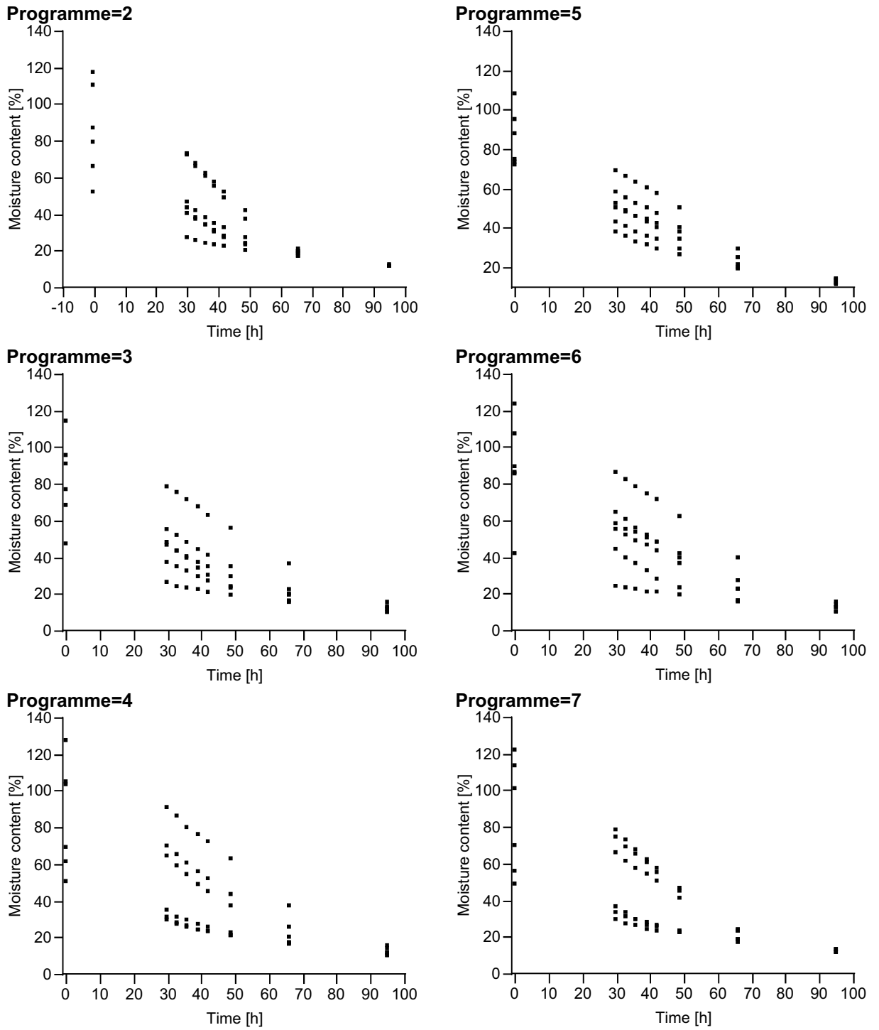
Figure 12. Moisture content over time for six samples in each of the six programs.
